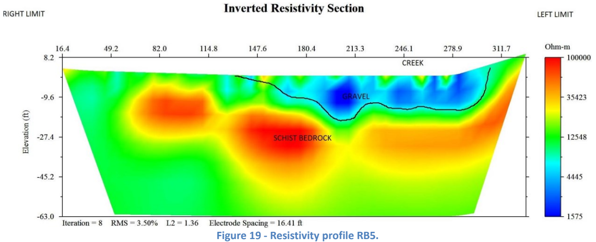
Figure 19 - Resistivity profile RB5.
