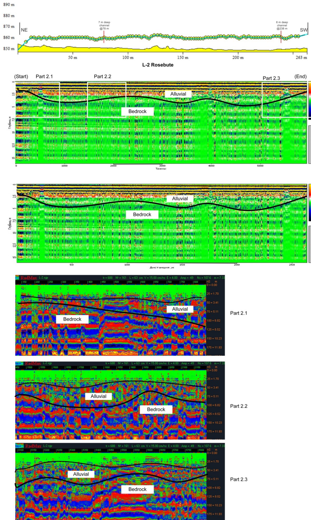
Figure 22 - Ground Penetrating Radar Line 2, Rosebute Creek.
