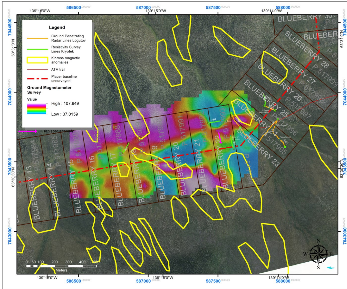
Figure 13 – Compilation map of 2016 exploration program on Rosebute Creek, showing Kinross regional magnetic anomalies (Hollis, 2011) overlain on the 2016 ground magnetometer survey. The locations of the ground penetrating radar lines and resistivity survey lines are also shown.
