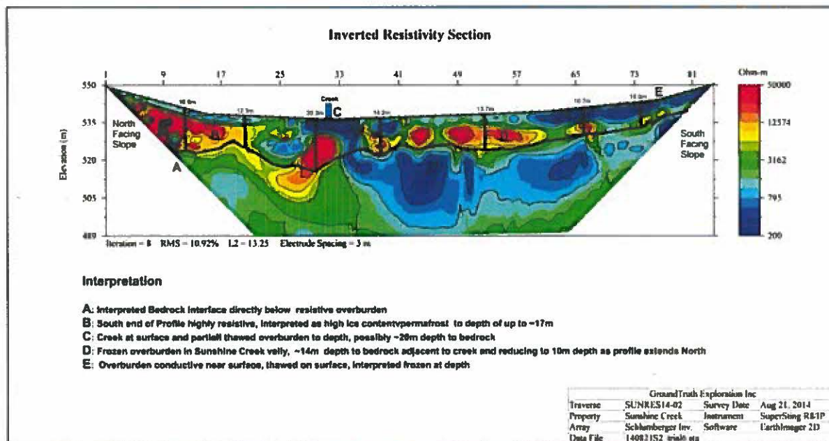
Figure 8: SUNRES14-02 Inverted Resistivity Interpretation
