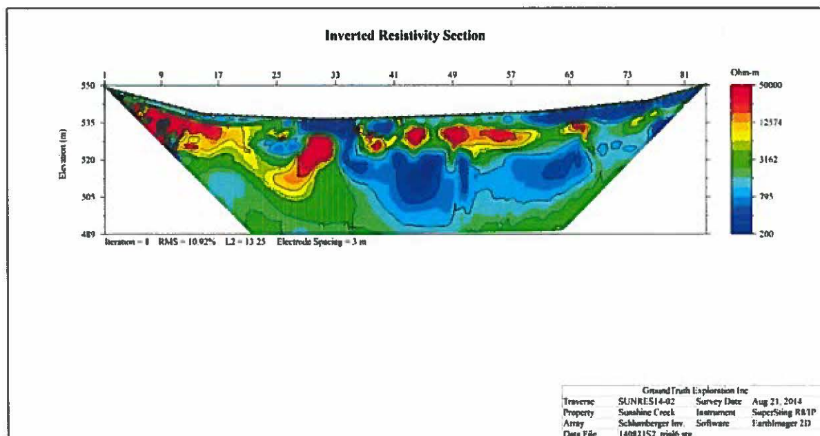
Figure 6: SUNRES14-02 Inverted Resistivity
