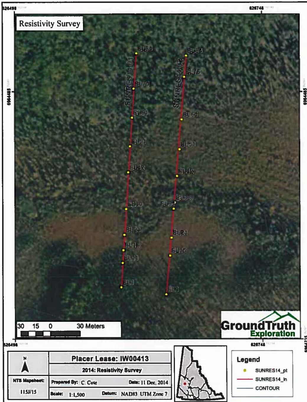
Figure 3: DC Resistivity Survey Location - Airphoto
