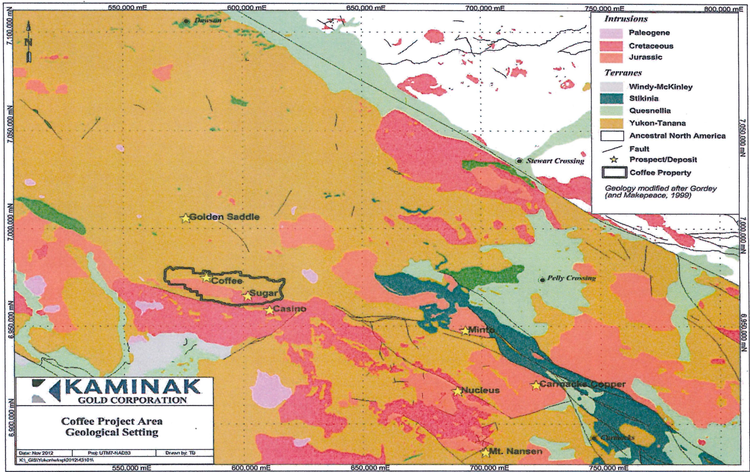
Figure 4-1: Geological Setting of the Coffee Project Area
