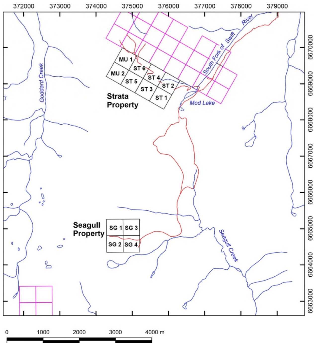
Figure 11a. Map showing location of Strata property and Seagull Property (both properties registered to Glen Prior). Other claims shown in magenta. Roads (trails) shown in red. Coordinates: UTM, NAD83, Zone 9V.
