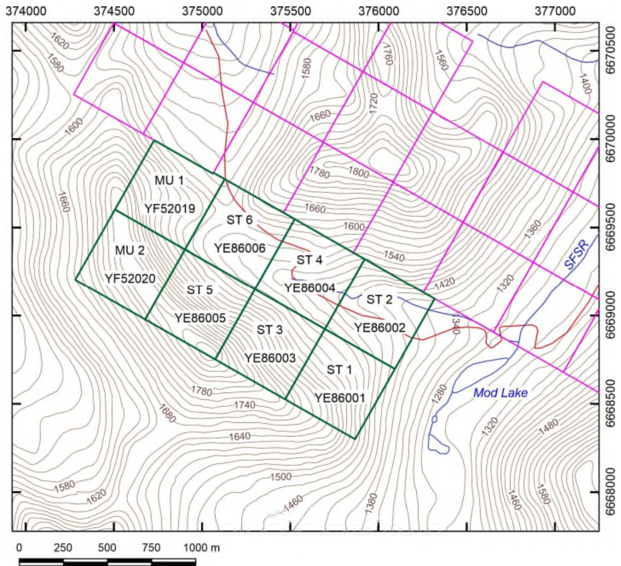
Figure 11b. Map of Strata property (green claim boundaries). Other claims shown in magenta. SFSR = South Fork of Swift River. Roads (trails) shown in red. Contour interval is 20 m. Coordinates: UTM, NAD83, Zone 9V.
