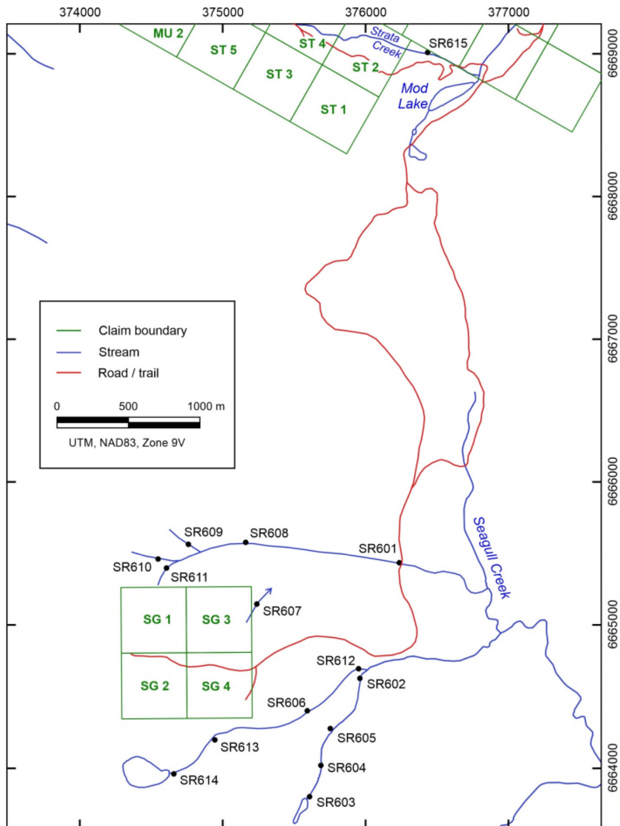
Figure 12. Map showing 2019 stream silt sample sites and sample numbers in the project area.
