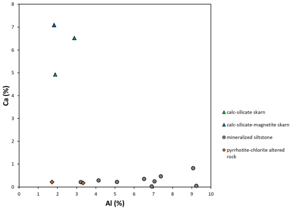
Figure 24. Binary plot of Al (four acid–ICP–MS) versus Ca (four acid–ICP–AES) showing rock sample data from the ST 5 area (values in weight percent).
