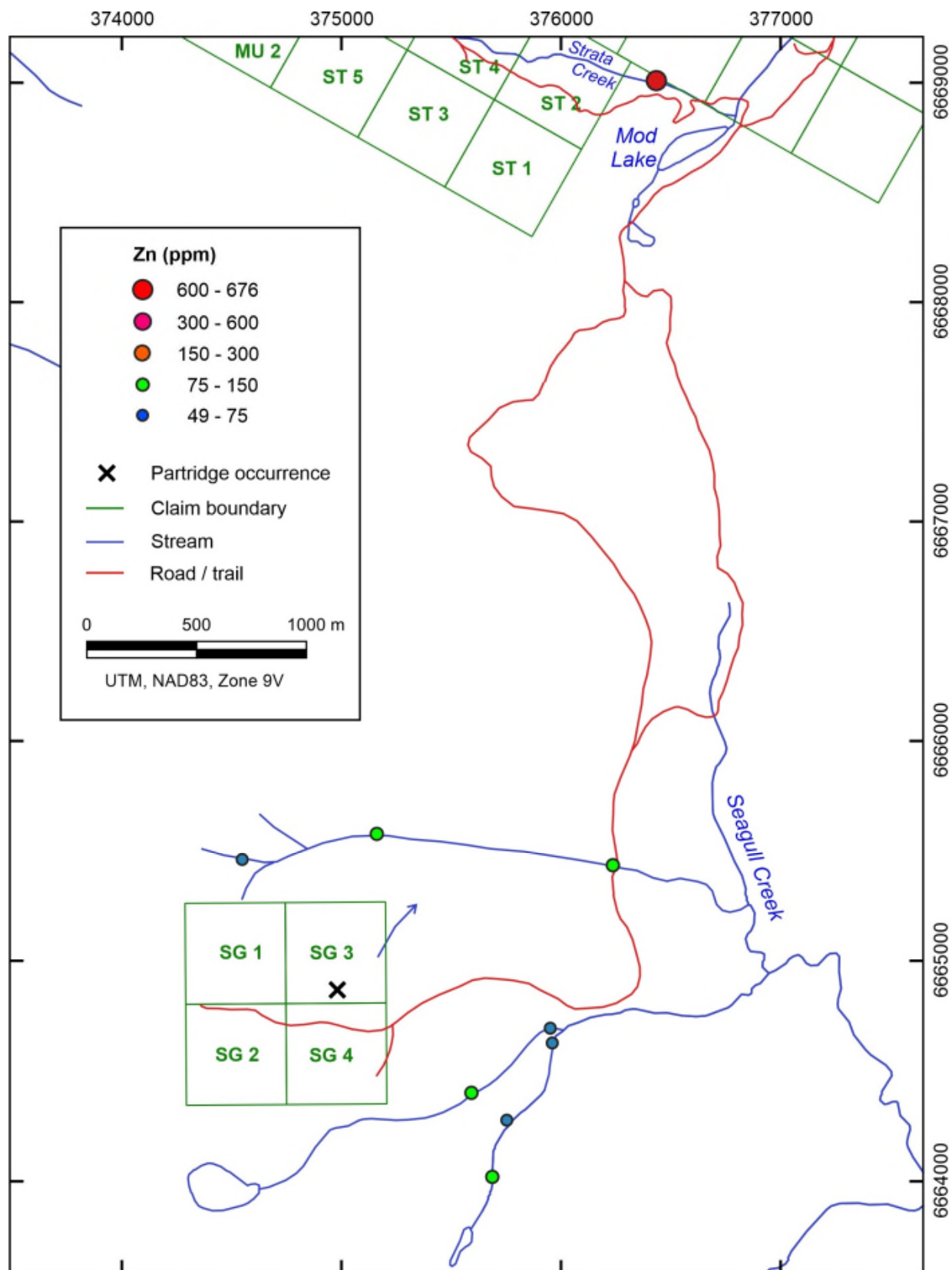
Figure 15. Map of zinc in 2019 heavy mineral concentrate samples.
