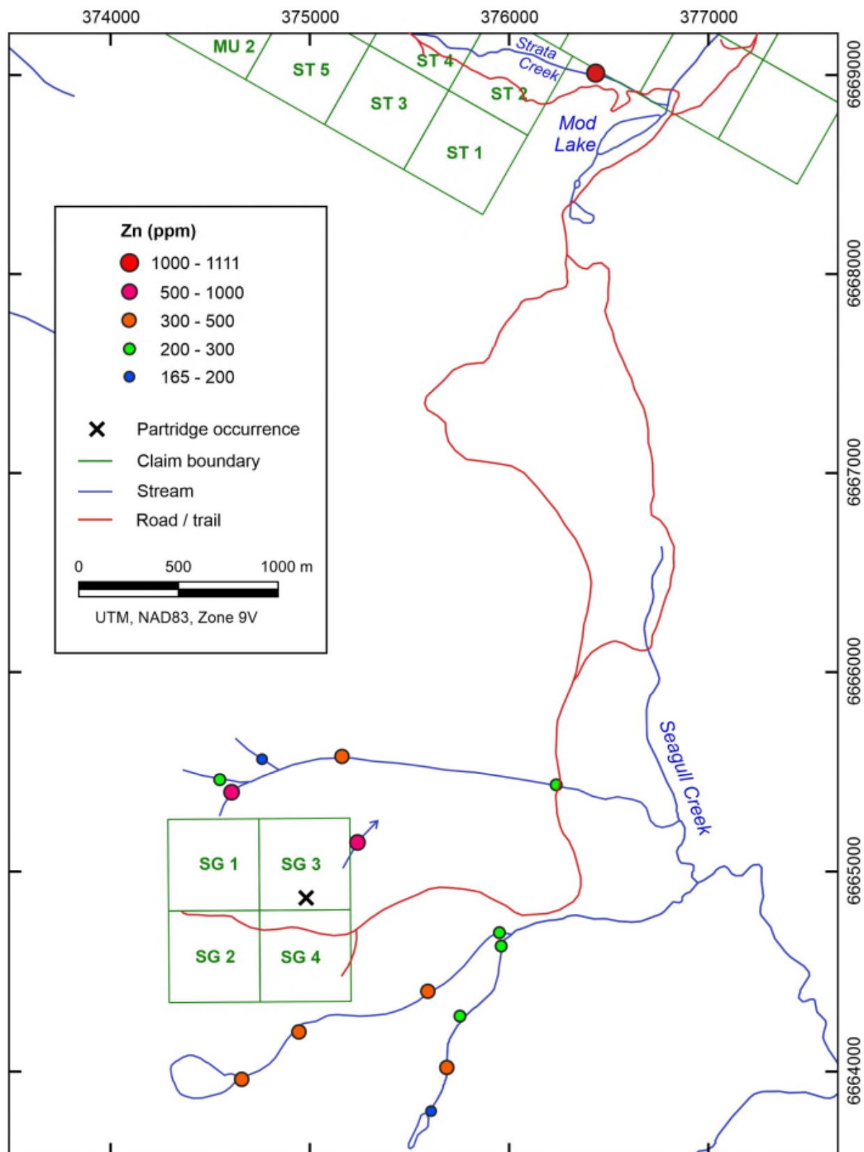
Figure 13. Map of zinc in 2019 stream silt samples.
