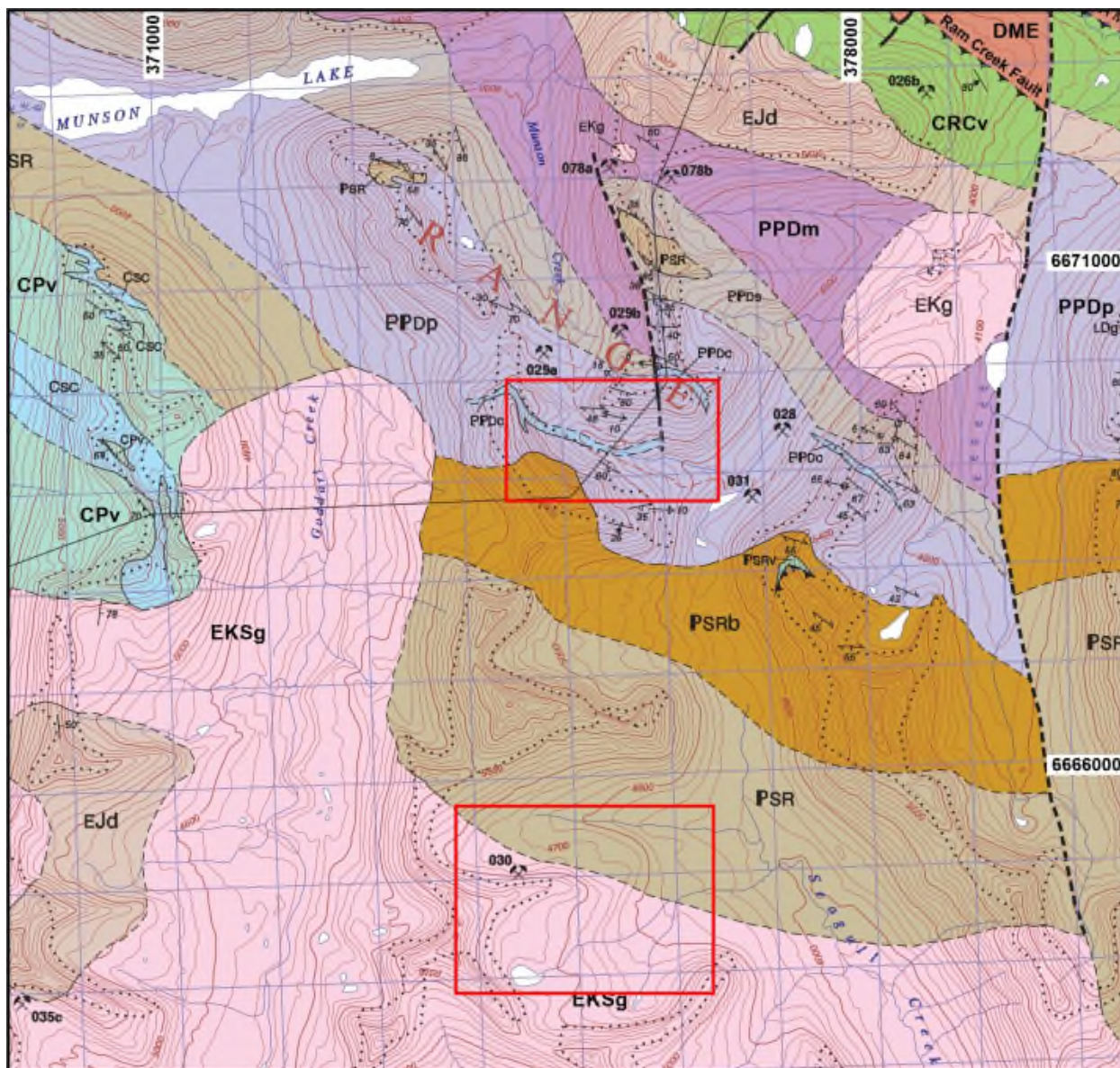
Figure 6a. Geology map of the central part of NTS map area 105B/03 (Roots et al., 2004). Exploration areas (2019) shown by rectangles with red perimeters: Rusty Valley area (which includes the Strata property) to the north and Partridge occurrence area to the south). Coordinates: UTM, NAD83, Zone 9V.
