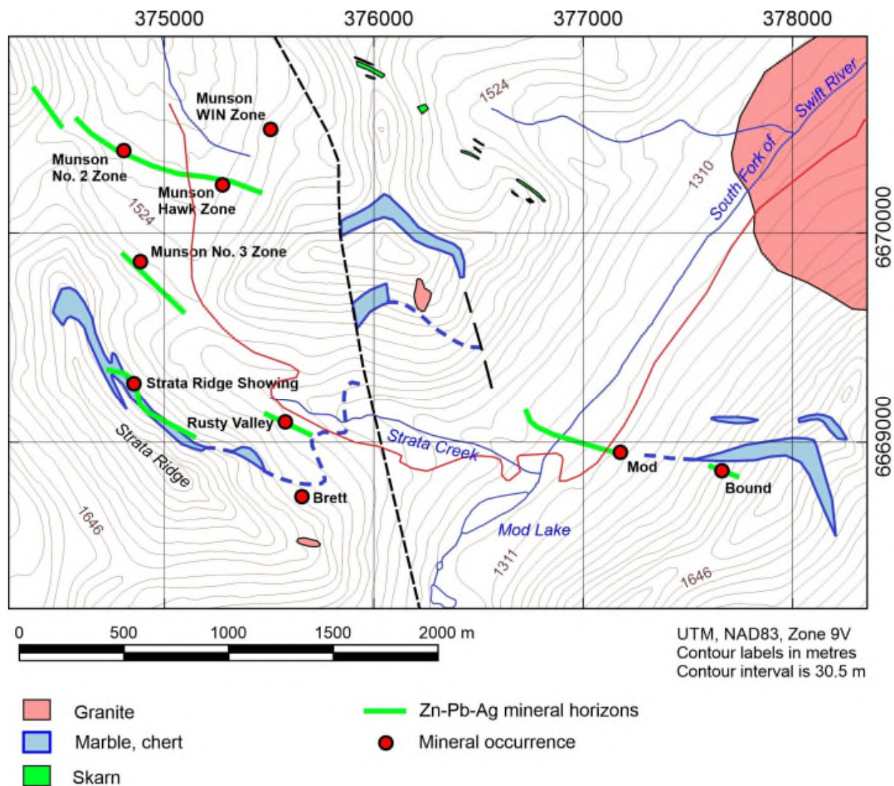
Figure 8. Map of the Rusty Valley (Strata Creek) area showing selected geological features. Distribution of granite and marble from Liverton and Casselman (2018). Distribution of skarn from Hodgson (1978). Distribution of Zn-Pb-Ag mineral horizons from Pautler (2007). Road (trail) shown in red.
