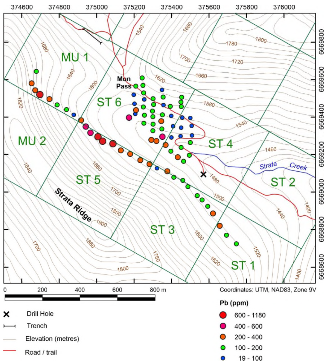
Figure 19. Map showing lead values in Strata property 2019 soil and talus fine-fraction samples. Claim boundaries and claim names shown in green (Strata property – ST and MU claims). The locations Trench 3 (northwest of Mun Pass) and the collar of diamond drill hole RV #1 are shown.
