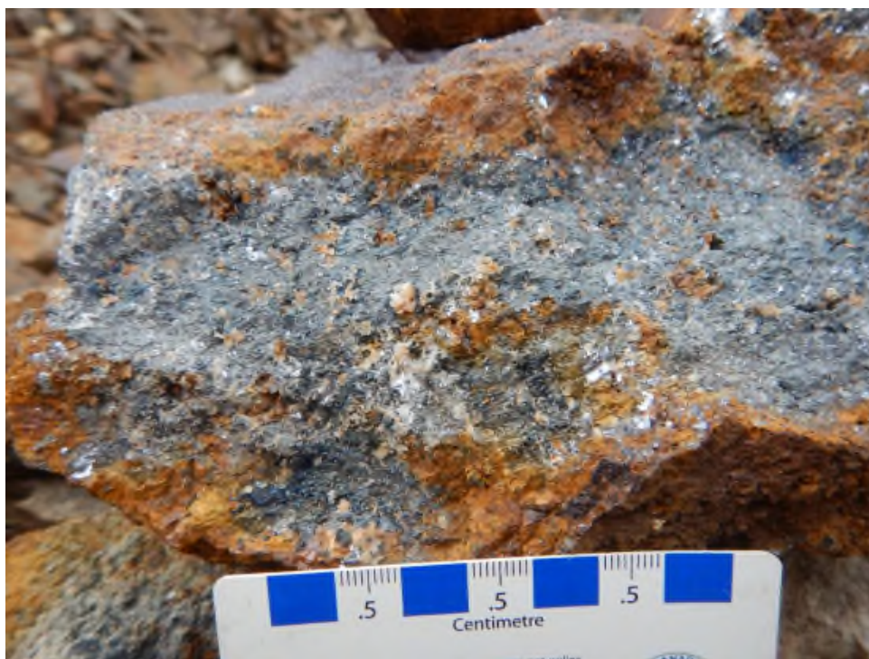
Figure 27. Photo showing Trench 3 rubble block from which sample SR424 was collected (21.37% Pb, 16.19% Zn and 356.8 g/t Ag). Photo taken at 374948E, 6669855N (UTM NAD83 Zone 9V).
