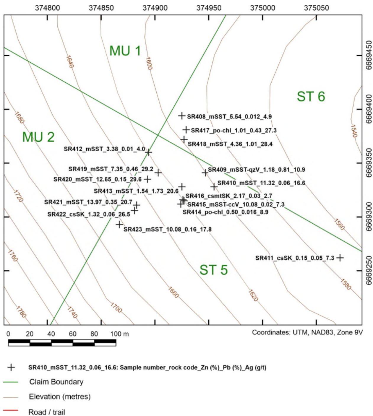
Figure 22. Map showing 2019 rock sample locations in the ST 5 area (Strata Ridge talus slope) along with Zn, Pb and Ag values. Rock codes: csSK = calc-silicate skarn, csmtSK = calc-silicate-magnetite skarn, mSST = mineralized siltstone, po-chl = pyrrhotite-chlorite altered rock, ccV = calcite veins, qzV = quartz vein.
