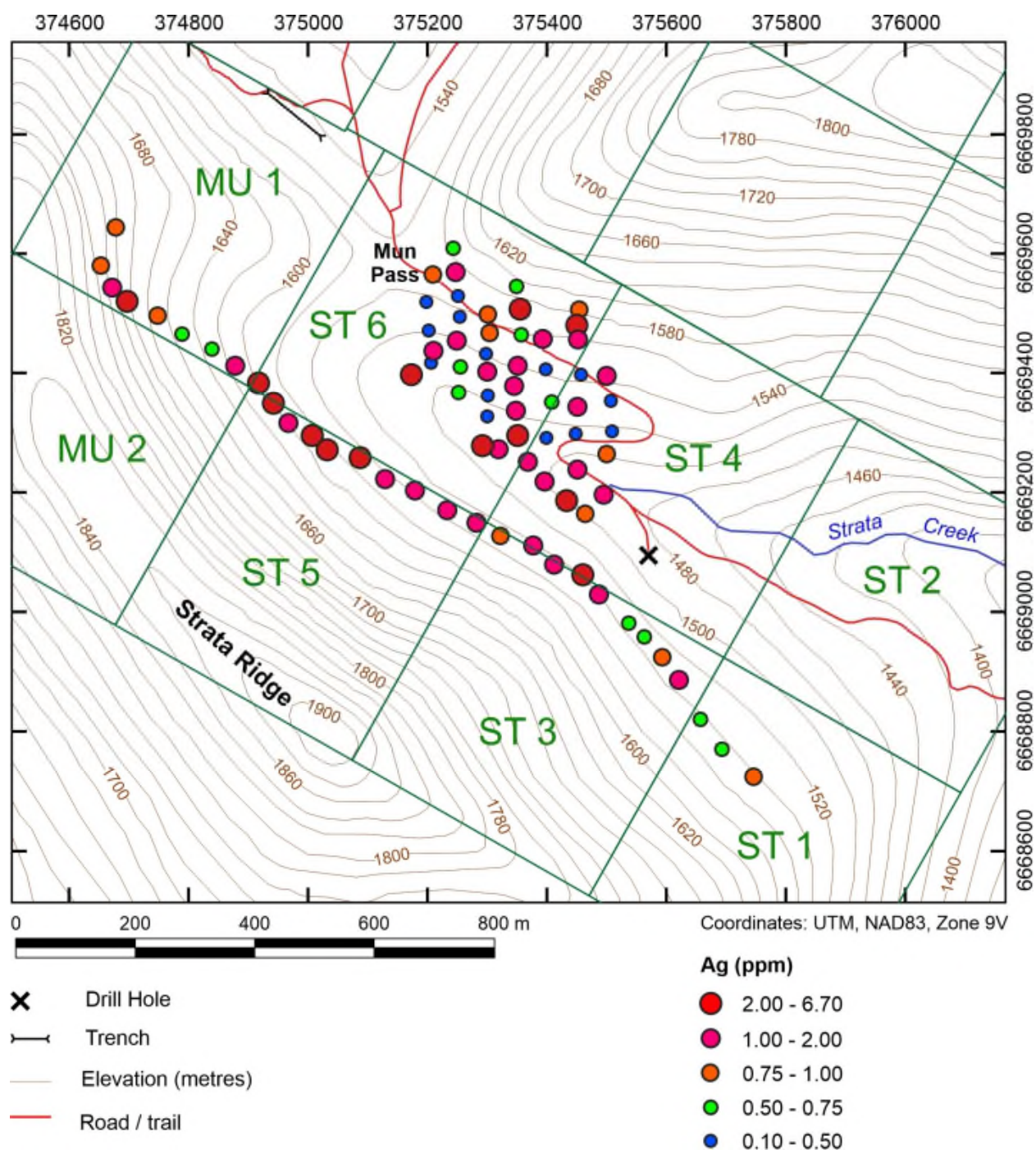
Figure 20. Map showing silver values in Strata property 2019 soil and talus fine-fraction samples. Claim boundaries and claim names shown in green (Strata property – ST and MU claims). The locations Trench 3 (northwest of Mun Pass) and the collar of diamond drill hole RV #1 are shown.
