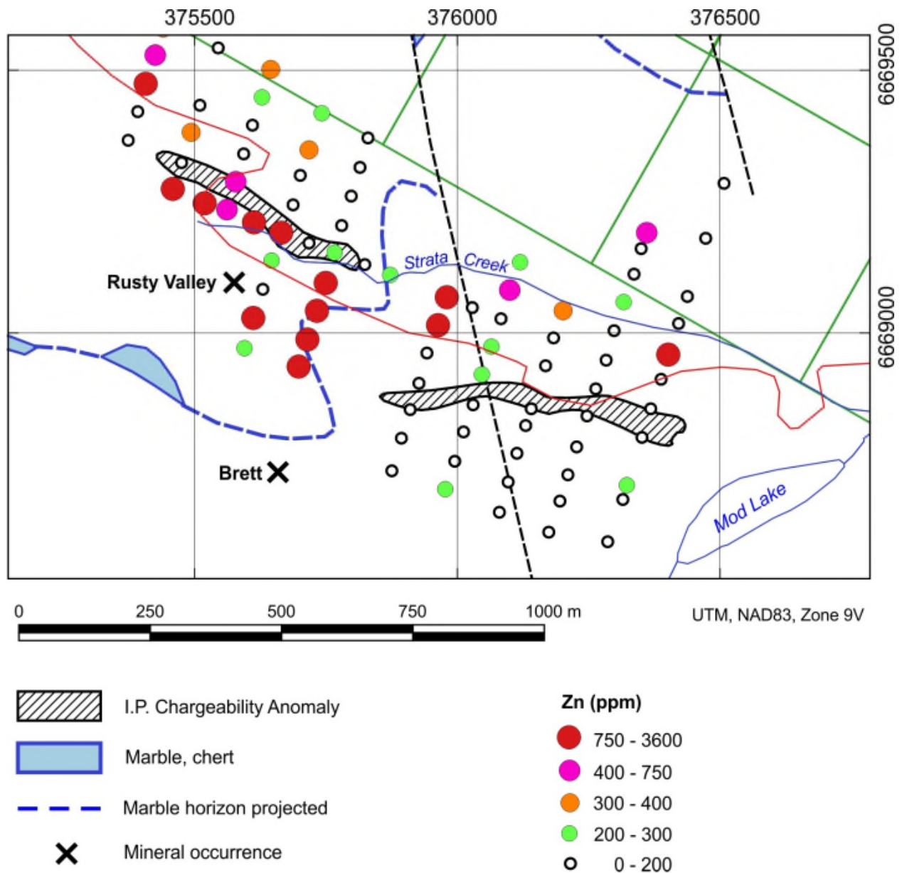
Figure 9. Zinc soil survey in the Rusty Valley (Strata Creek) area (soil and I.P. data from McLeod and Sevensma, 1969). Distribution of marble is from Liverton and Casselman (2018). The “X” marking the Rusty Valley occurrence is located at the collar location of holes RV #1 and RV #2. Quartz claims in good standing at the end of 2018 are shown in green. The road (trail) is shown in red.
