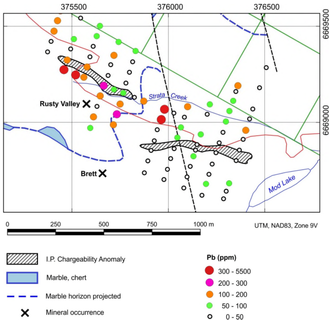
Figure 10. Lead soil survey in the Rusty Valley (Strata Creek) area (soil and I.P. data from McLeod and Sevensma, 1969). Distribution of marble is from Liverton and Casselman (2018). The “X” marking the Rusty Valley occurrence is located at the collar location of holes RV #1 and RV #2. Quartz claims in good standing at the end of 2018 are shown in green. The road (trail) is shown in red.
