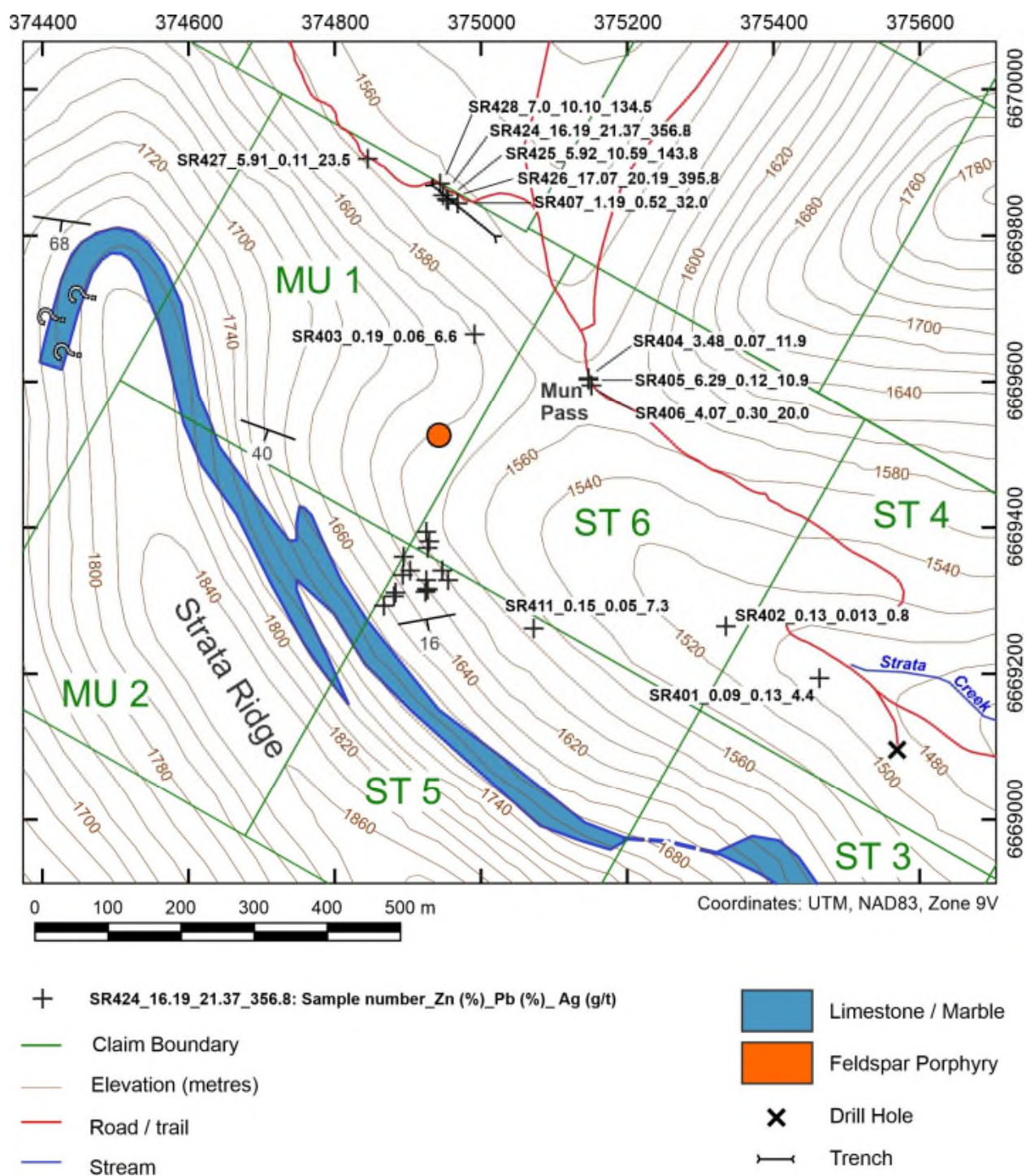
Figure 21. Map showing 2019 rock sample locations within the Strata property along with Zn, Pb and Ag values. See Figure 22 for information on cluster of samples on the northeast flank of Strata Ridge. The locations Trench 3 (northwest of Mun Pass) and the collar of diamond drill hole RV #1 are shown. The distribution of the limestone / marble unit is based on Liverton and Casselman (2018) and 2019 field observations in the northwest part of Strata Ridge. The feldspar porphyry unit is based on a single outcrop.
