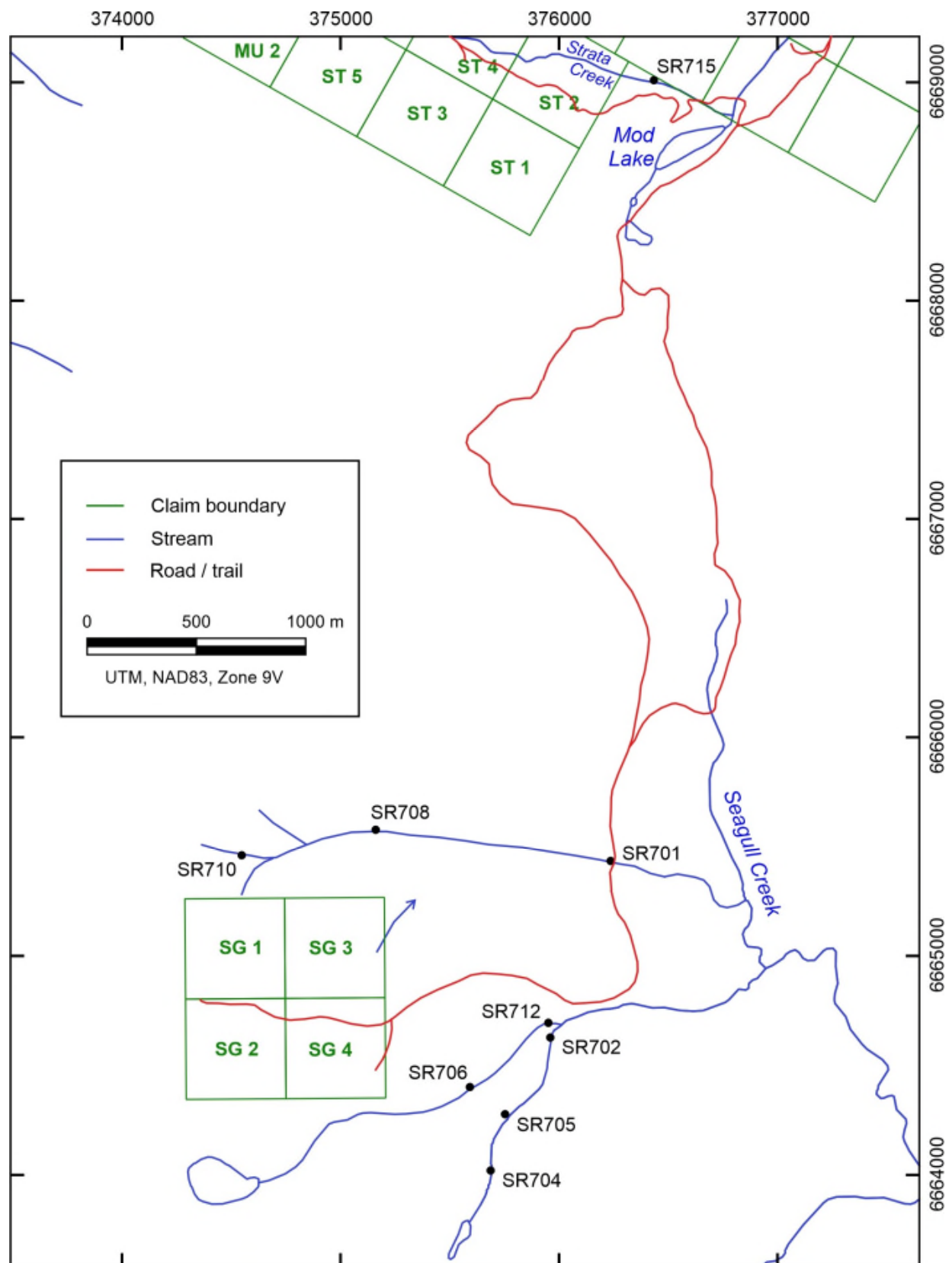
Figure 14. Map showing 2019 heavy mineral concentrate sample sites and numbers in the project area.
