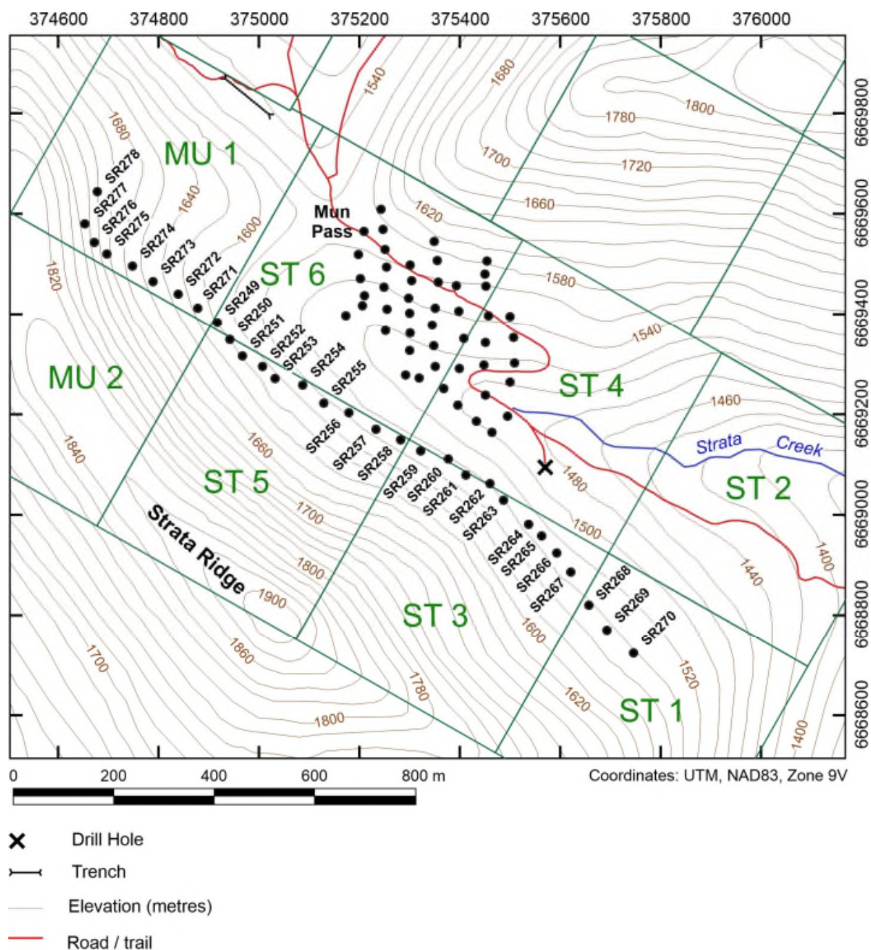
Figure 16. Map showing 2019 Strata property soil and talus fine-fraction sample sites. Talus fine-fraction samples collected from the middle to upper part of the talus slope on the eastern flank of Strata Ridge are labelled. Numbers for soil samples collected from the sampling grid within claims ST 4 and ST 6 are shown in Figure 17. Claim boundaries shown in green. The locations Trench 3 (northwest of Mun Pass) and the collar of diamond drill hole RV #1 are shown.
