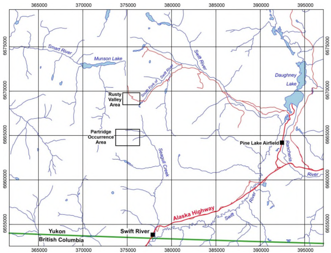
Figure 2. Location of the Swift River project exploration areas (rectangles with black perimeters). The Strata property lies within the Rusty Valley area. Coordinates: UTM, NAD 83, Zone 9V. Grid lines are 5 km apart.
