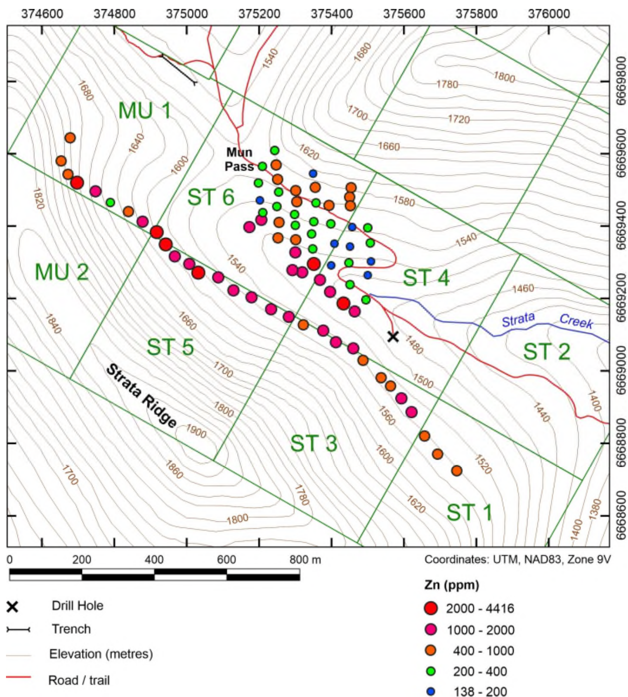
Figure 18. Map showing zinc values in 2019 Strata property soil and talus fine-fraction samples. Claim boundaries and claim names shown in green (Strata property = ST and MU claims). The locations Trench 3 (northwest of Mun Pass) and the collar of diamond drill hole RV #1 are shown.
