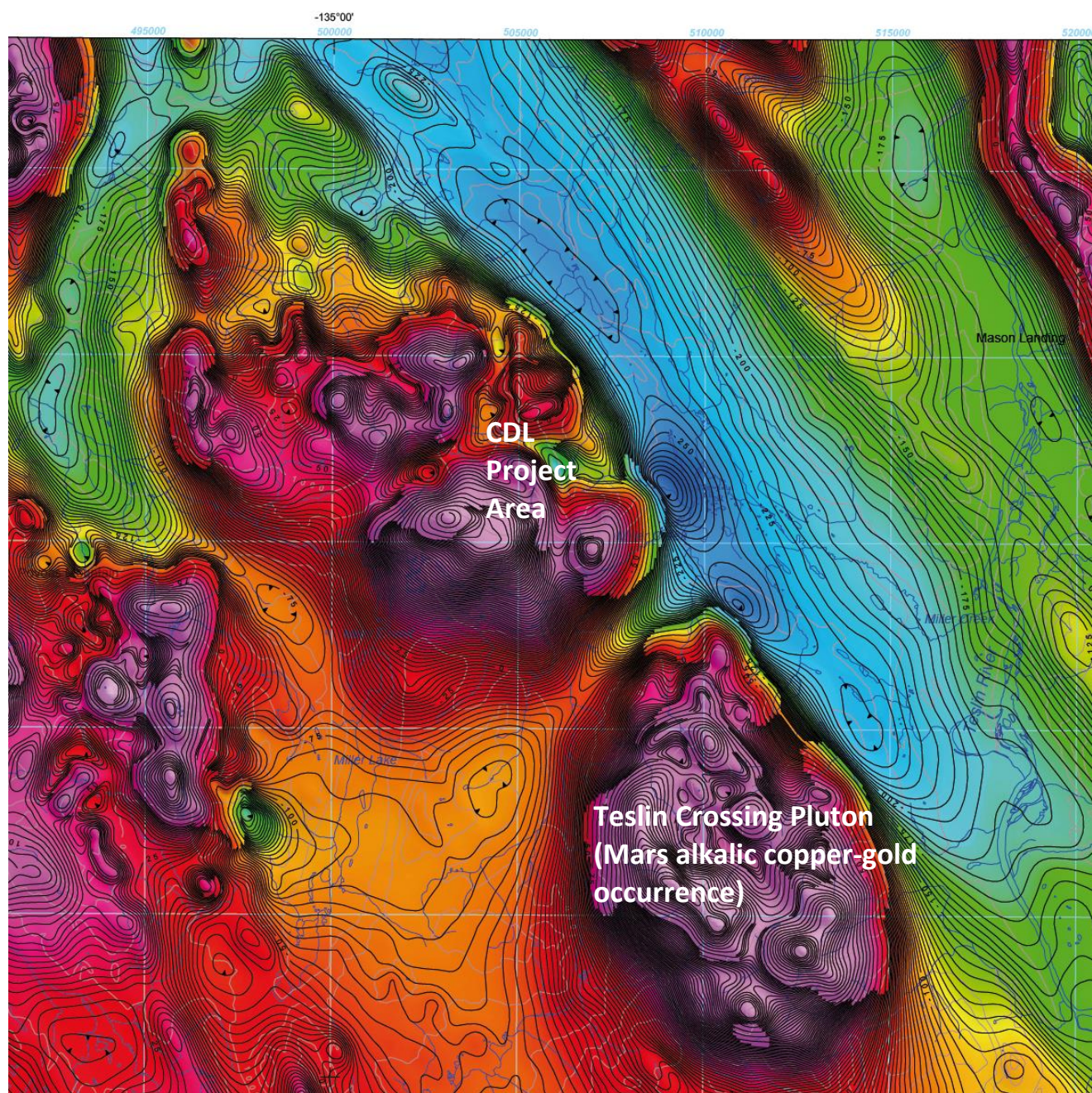
Figure 5 Aeromagnetic Survey Map
