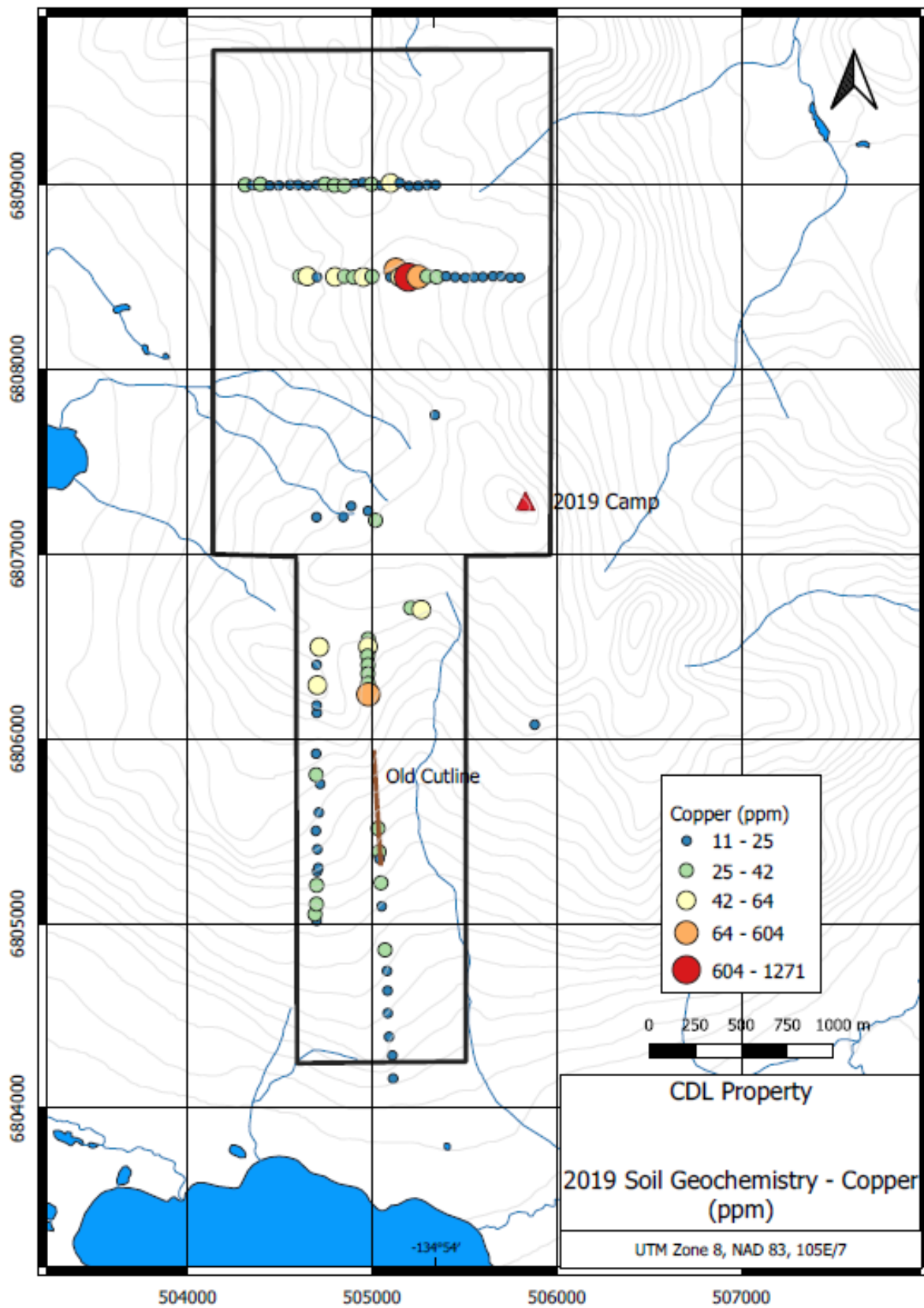
Figure 7 Soil Geochemistry - Copper (ppm)
