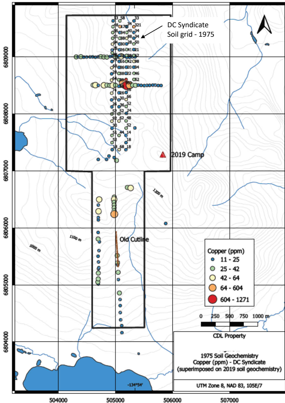
Figure 8 1975 Soil Geochemistry - Copper (DC Syndicate)
