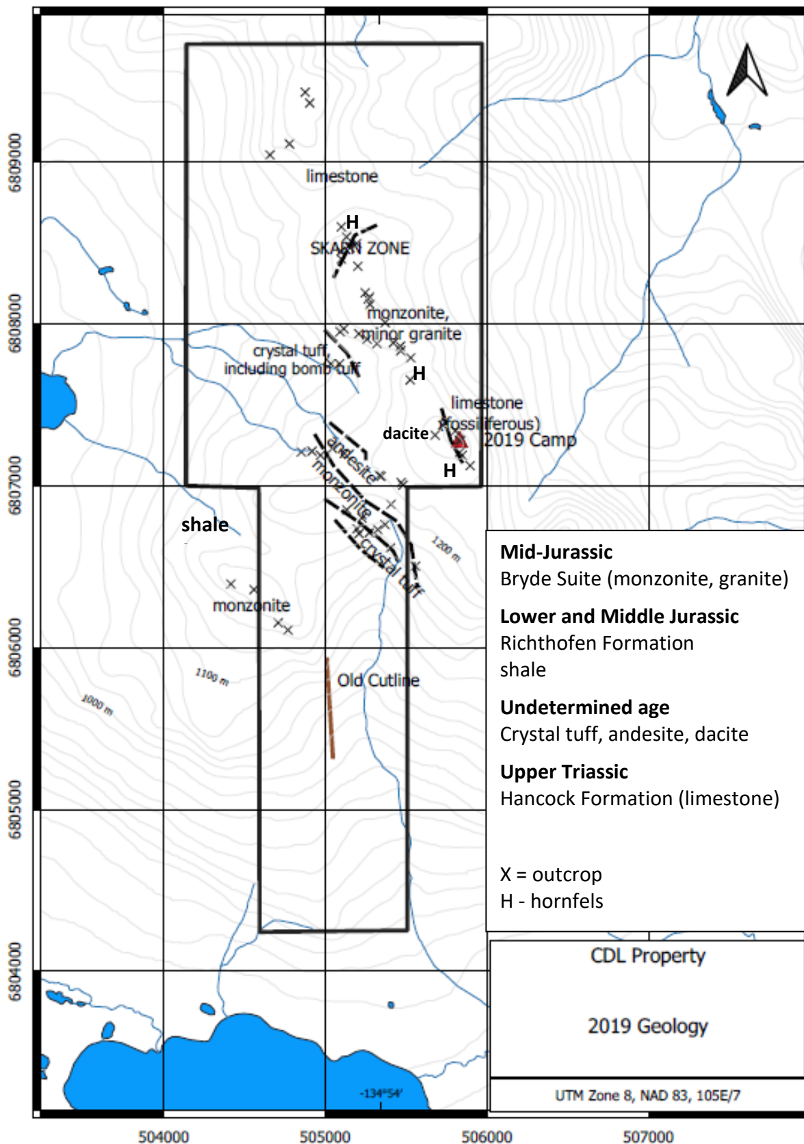
Figure 12 CDL Geology
