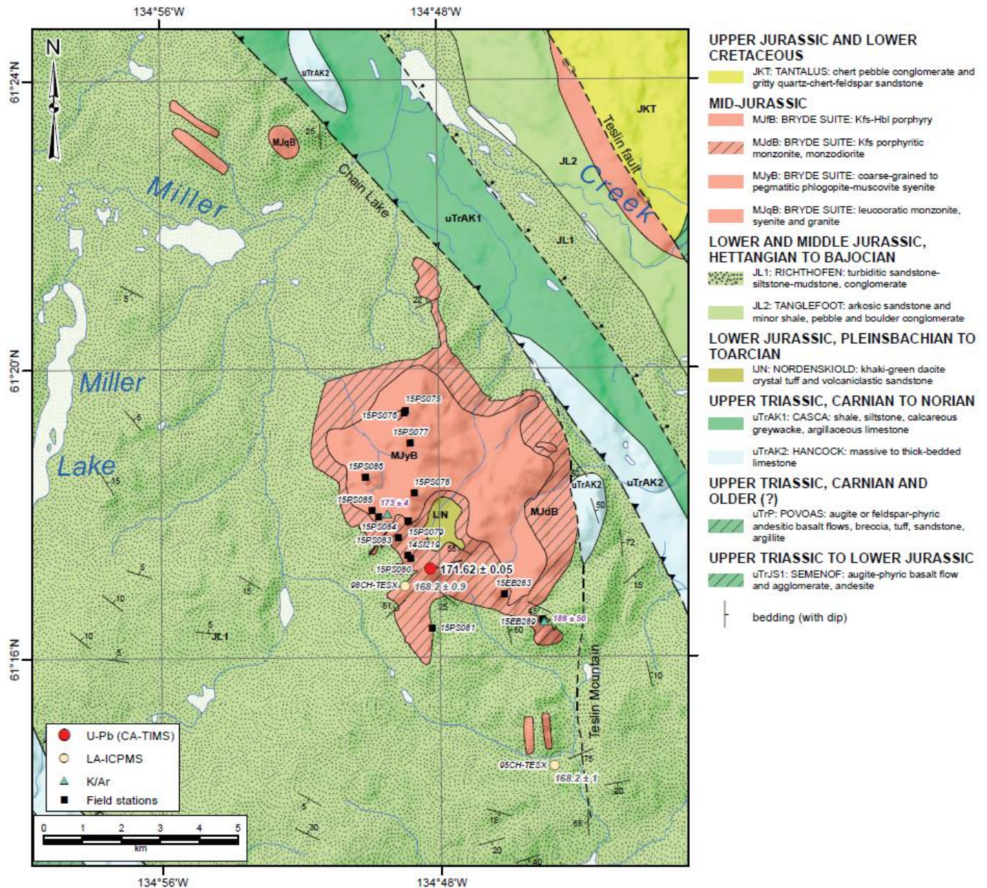
Figure 4 Regional Geology
