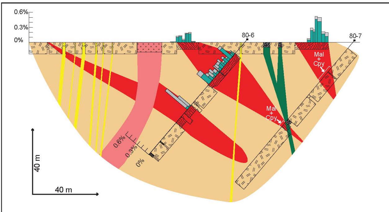
Figure 5-3: Cross section from Sack et al., 2016. Green (oxide) and grey (sulphide) bars are results from trenches or core reassayed in 2015. Hole 80-7 was not reassayed and mineralized zones are based on visible copper mineralization from original logs.
