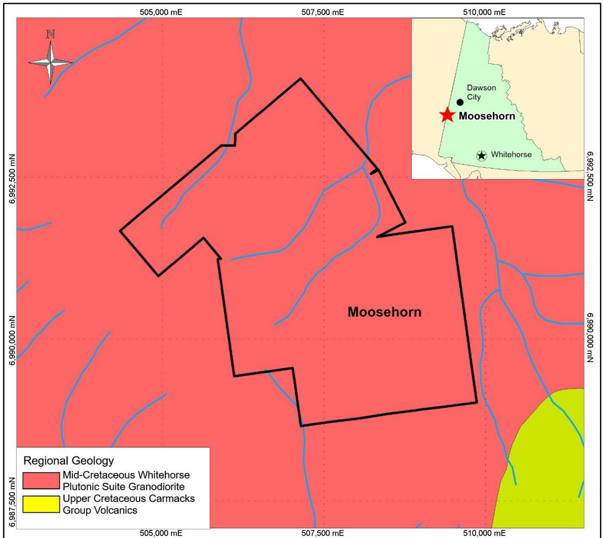
Figure 3 – Regional Geology
