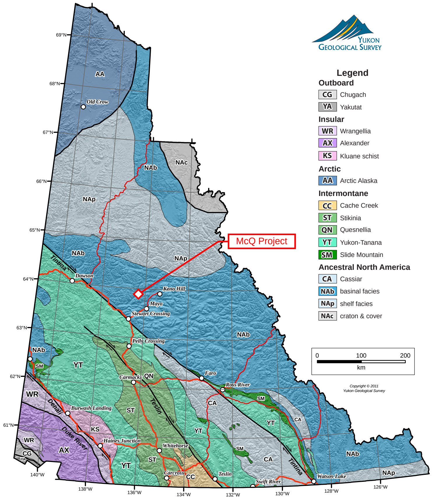
Figure 3 - Yukon Terrane Map
