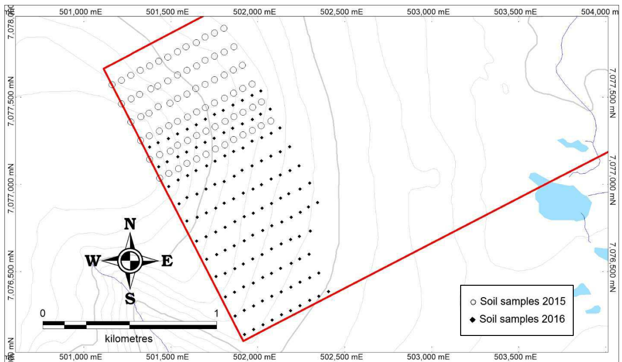
Figure 13: The Carlin grid with sample sites distinguished based on year of sampling
