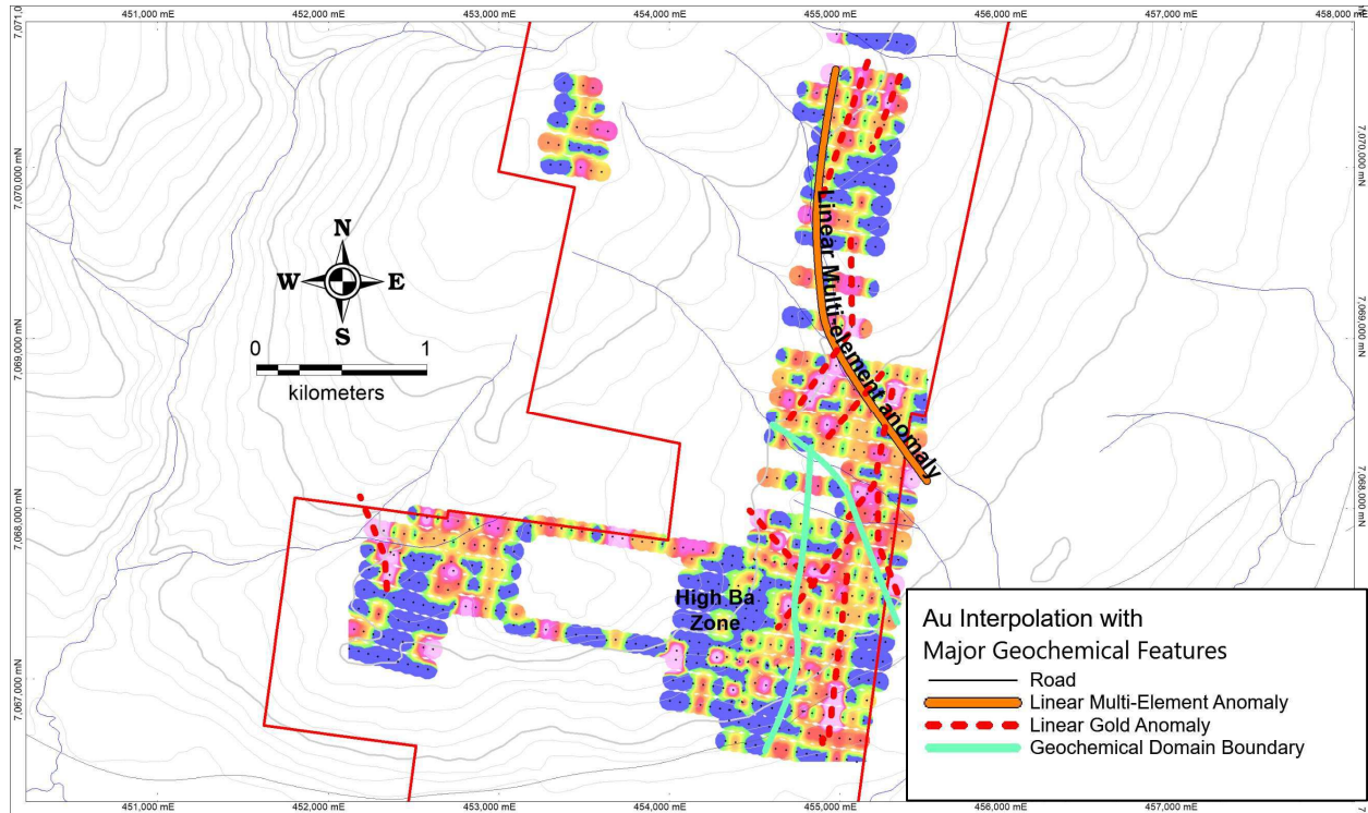
Figure 16: Roaring Fork grid with major geochemical anomalies and boundaries illustrated
