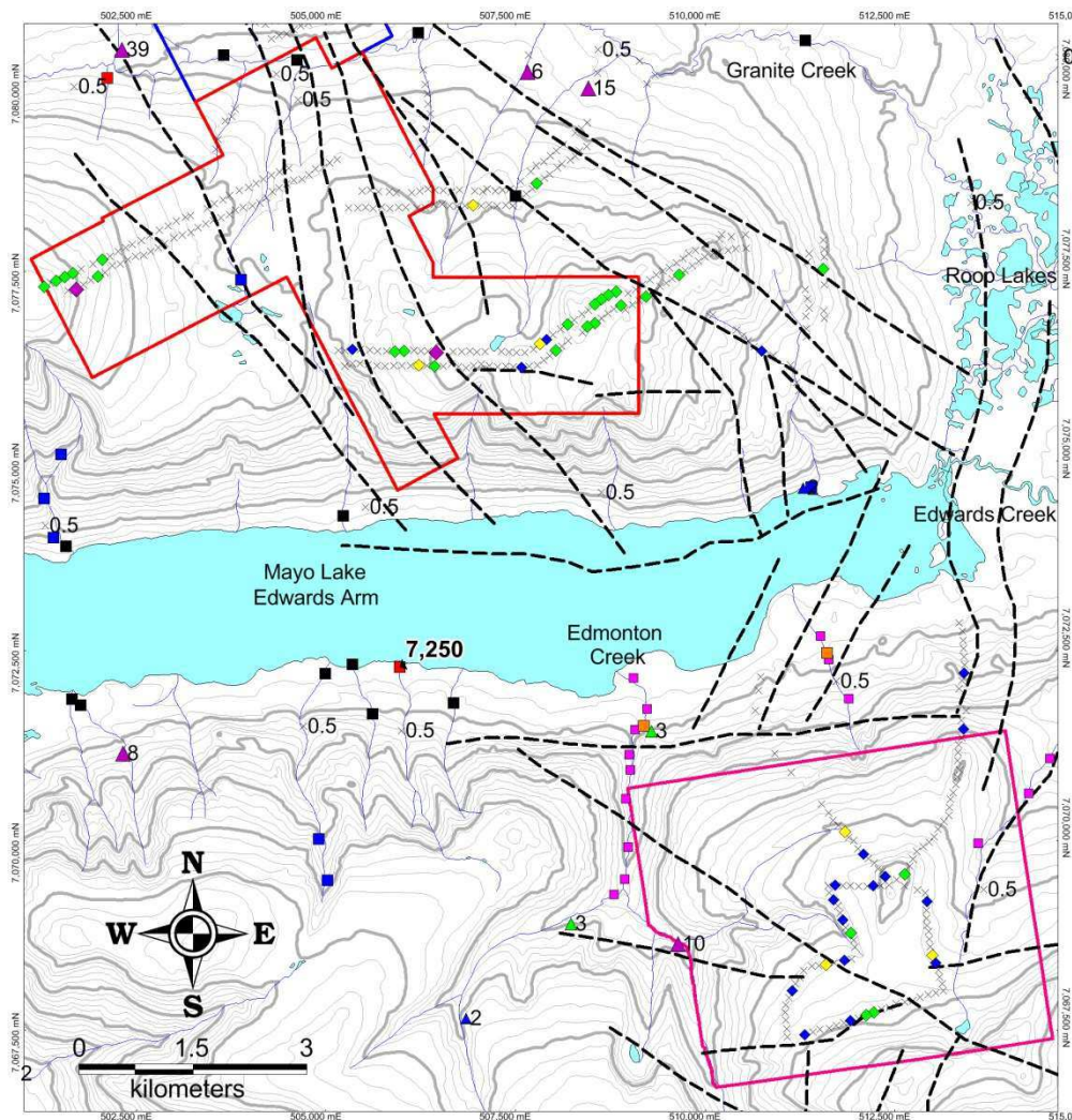
Figure 5: Previous work on the Edmonton and Carlin Claim Groups
