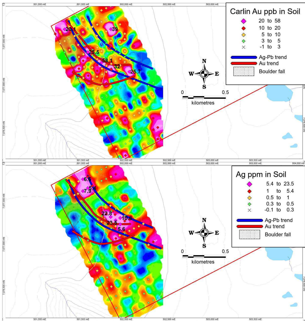
Figure 14: Interpolated Au in soil (above) and Ag in soil (below). Soil points show Au and Ag respectively
