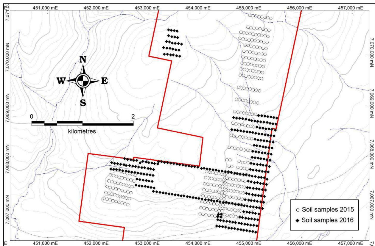
Figure 10: The Roaring Fork grid with sample sites distinguished based on year of sampling
