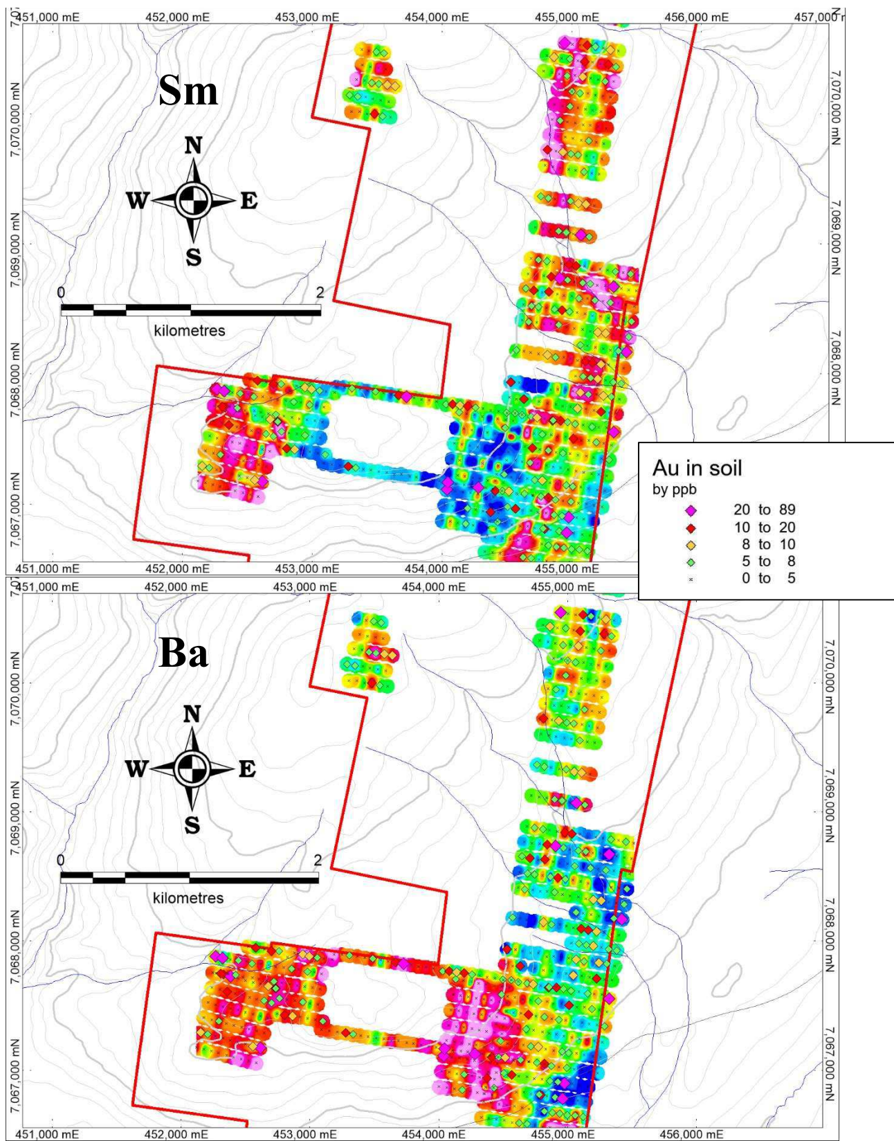
Figure 12: Interpolated Sm (above) and Ba (below) in soil from 2015 and 2016 sampling. Soil points show Au values at sample sites.
