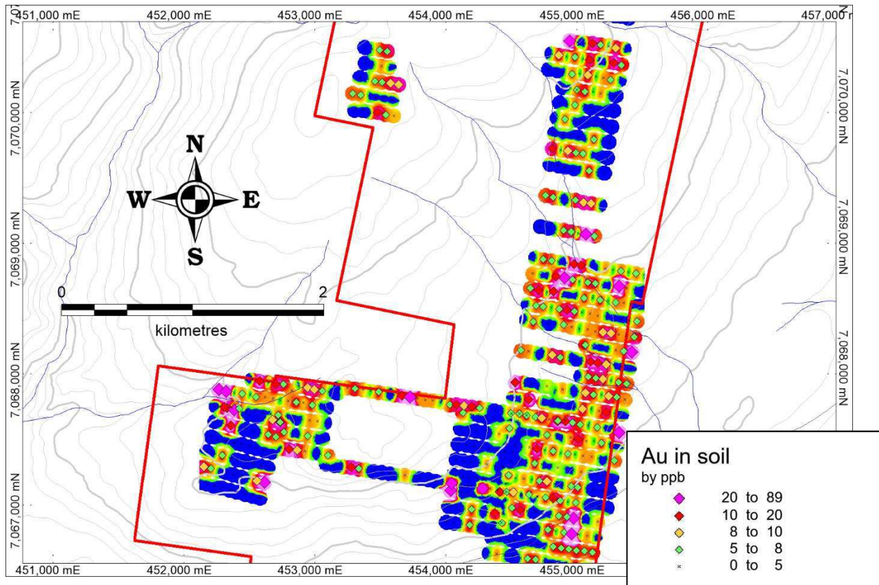
Figure 11: Interpolated Au in soil from 2015 and 2016 sampling
