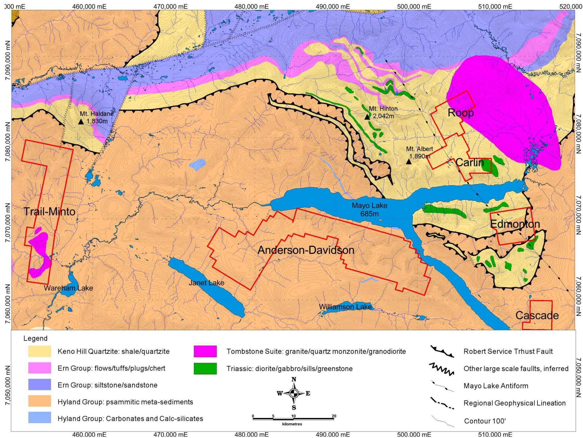
Figure 8: Geology of Mayo Lake showing MLM claim groups claim extents as of 2015.
