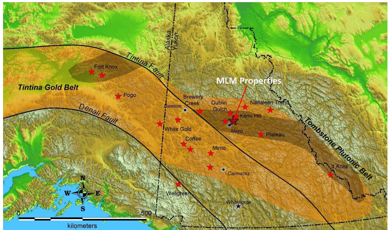
Figure 15: location of significant mines and deposits of the Selwyn basin as related to Fort Knox
