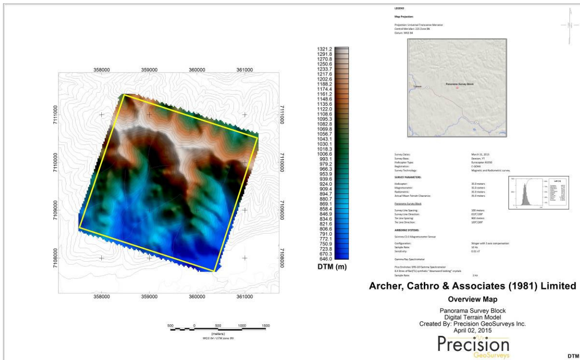
Map 2: Panorama survey block digital terrain model.
