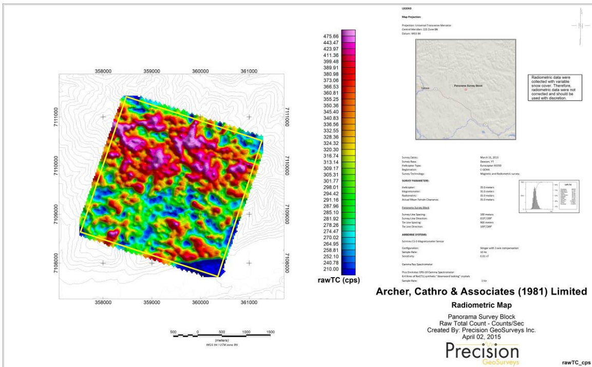
Map 10: Panorama survey block raw total count – counts/sec
