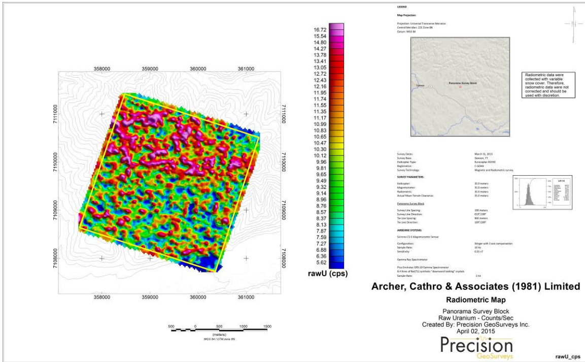
Map 9: Panorama survey block raw uranium – counts/sec.
