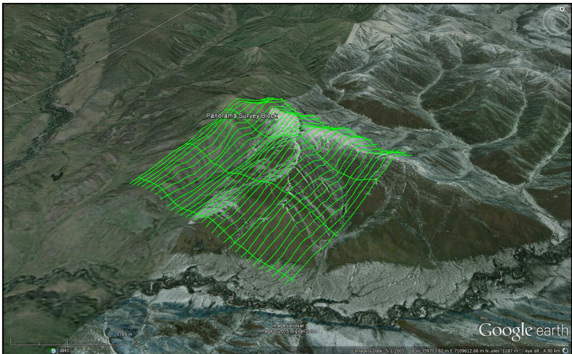
Figure 4: Terrain View – Panorama survey block with actual survey and tie lines displayed in green.
