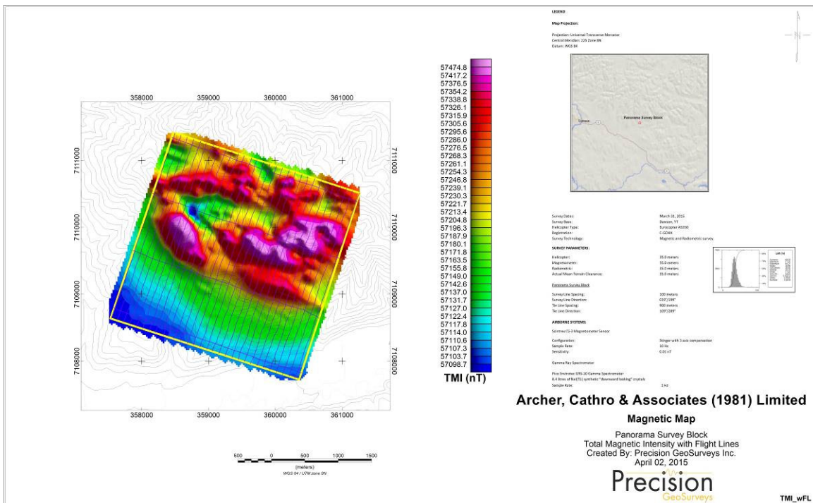
Map 4: Panorama survey block total magnetic intensity with displayed actual flight lines.
