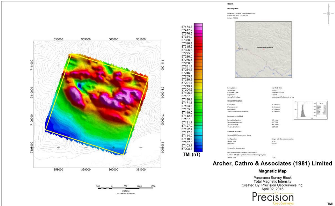
Map 3: Panorama survey block total magnetic intensity.
