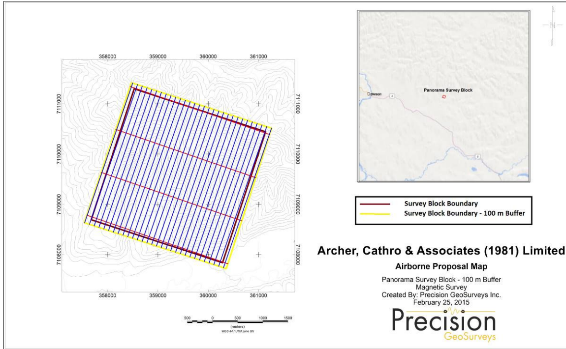
Figure 5: Survey map of Panorama survey area with 100 m buffer zone showing proposed survey and tie lines. The survey block boundary outline in brown and the 100 m buffer zone outline in yellow.
