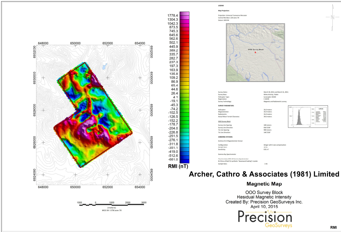
Map 5: OOO survey block residual magnetic intensity.
