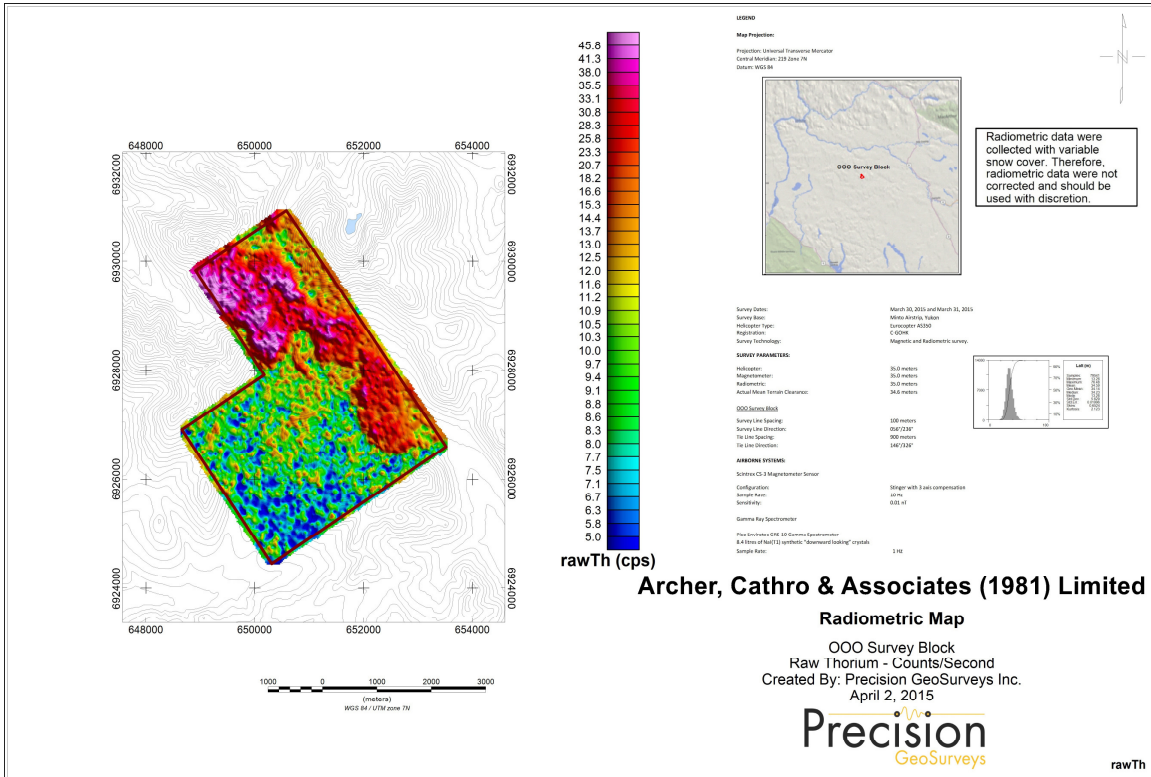
Map 8: OOO survey block raw thorium – counts/sec.
