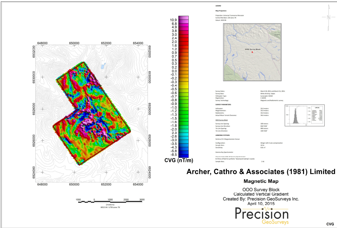
Map 6: OOO survey block calculated vertical gradient of the total magnetic intensity.
