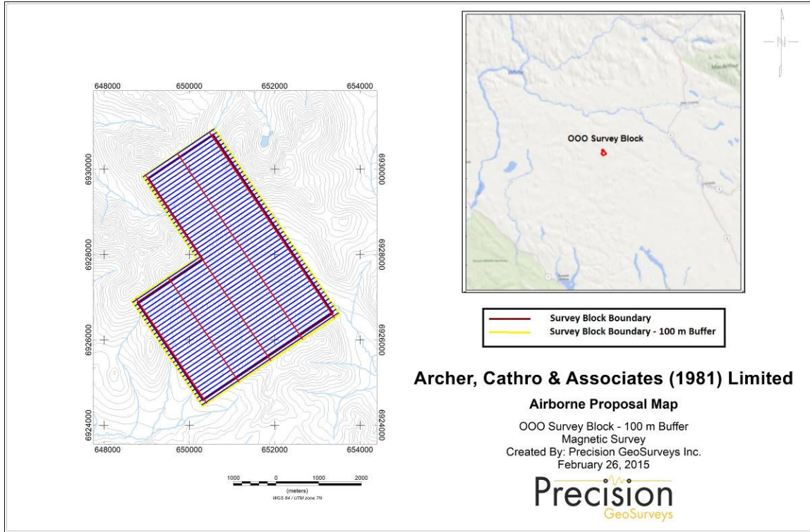
Figure 5: Survey map of OOO survey area with 100 m buffer zone showing proposed survey and tie lines. The survey block boundary outline in brown and the 100 m buffer zone outline in yellow.
