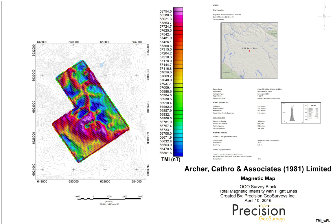
Map 4: OOO survey block total magnetic intensity with displayed actual flight lines.
