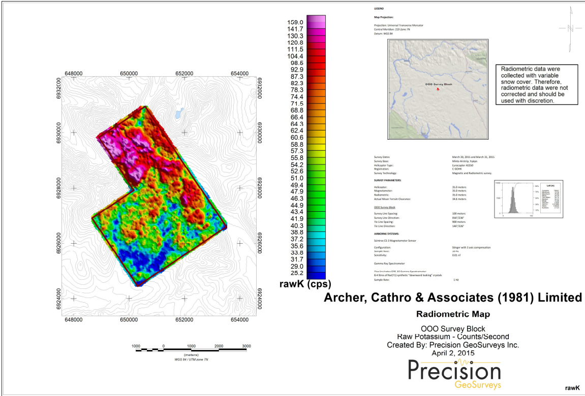
Map 7: OOO survey block raw potassium – counts/sec.
