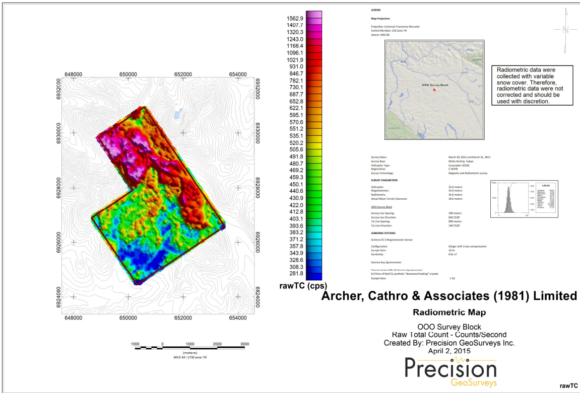
Map 10: OOO survey block raw total count – counts/sec
