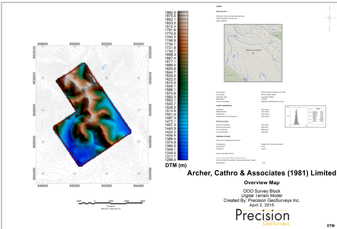
Map 2: OOO survey block digital terrain model.
