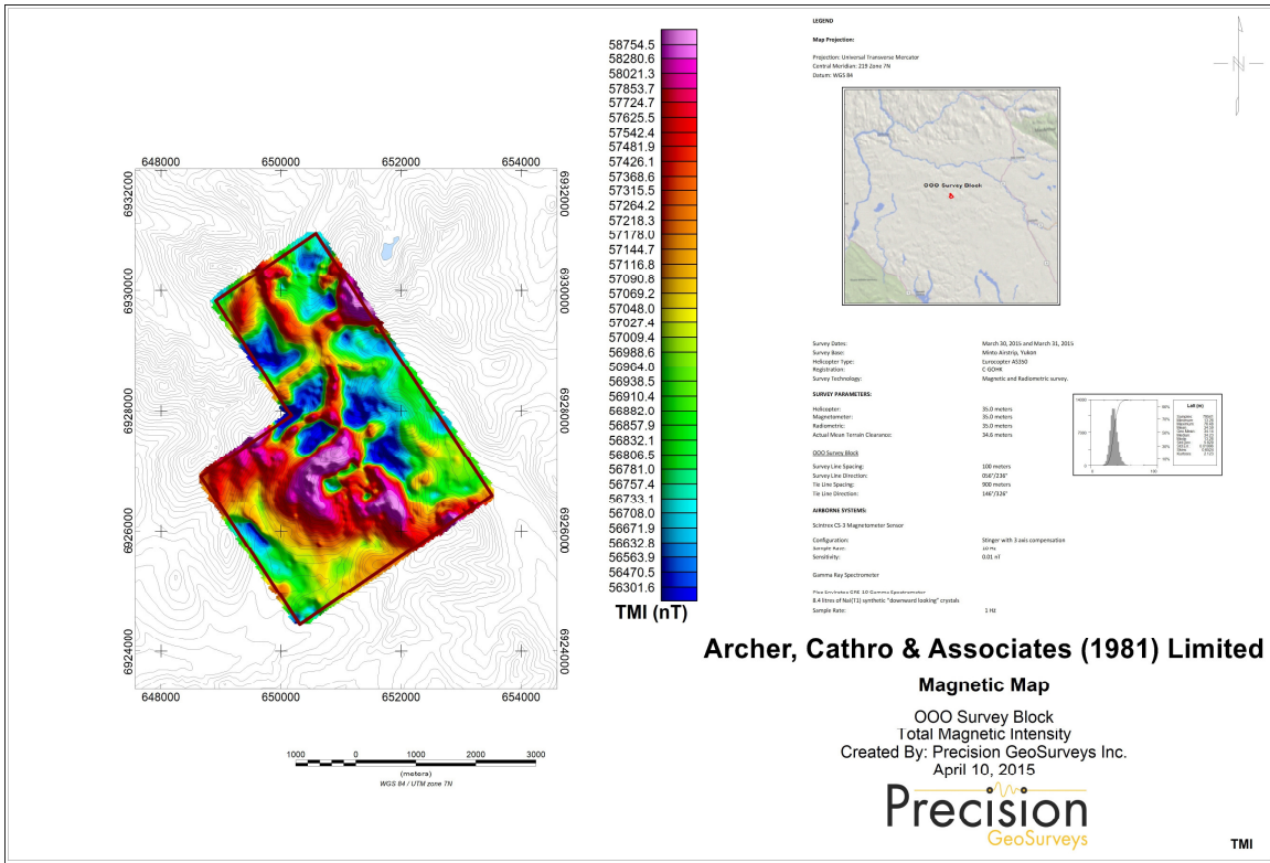
Map 3: OOO survey block total magnetic intensity.
