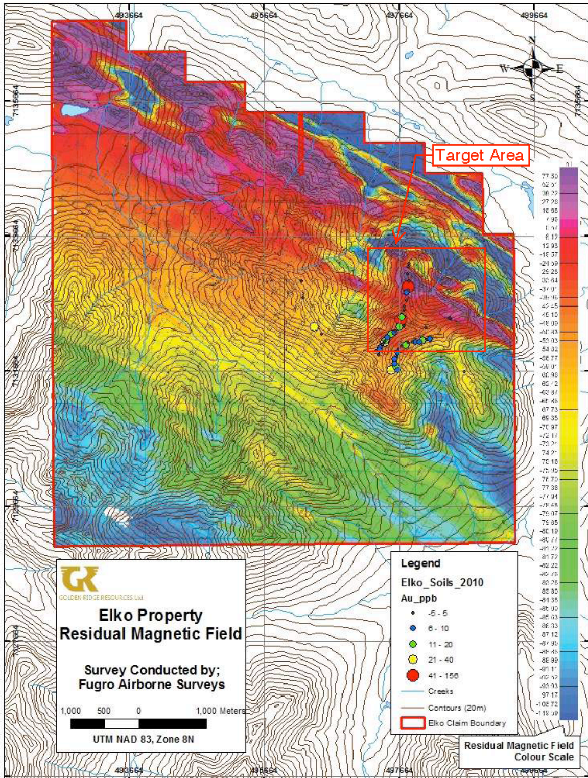
Figure 8. Residual magnetic field and 2010 gold in soil values (from Piepgrass, 2012).
