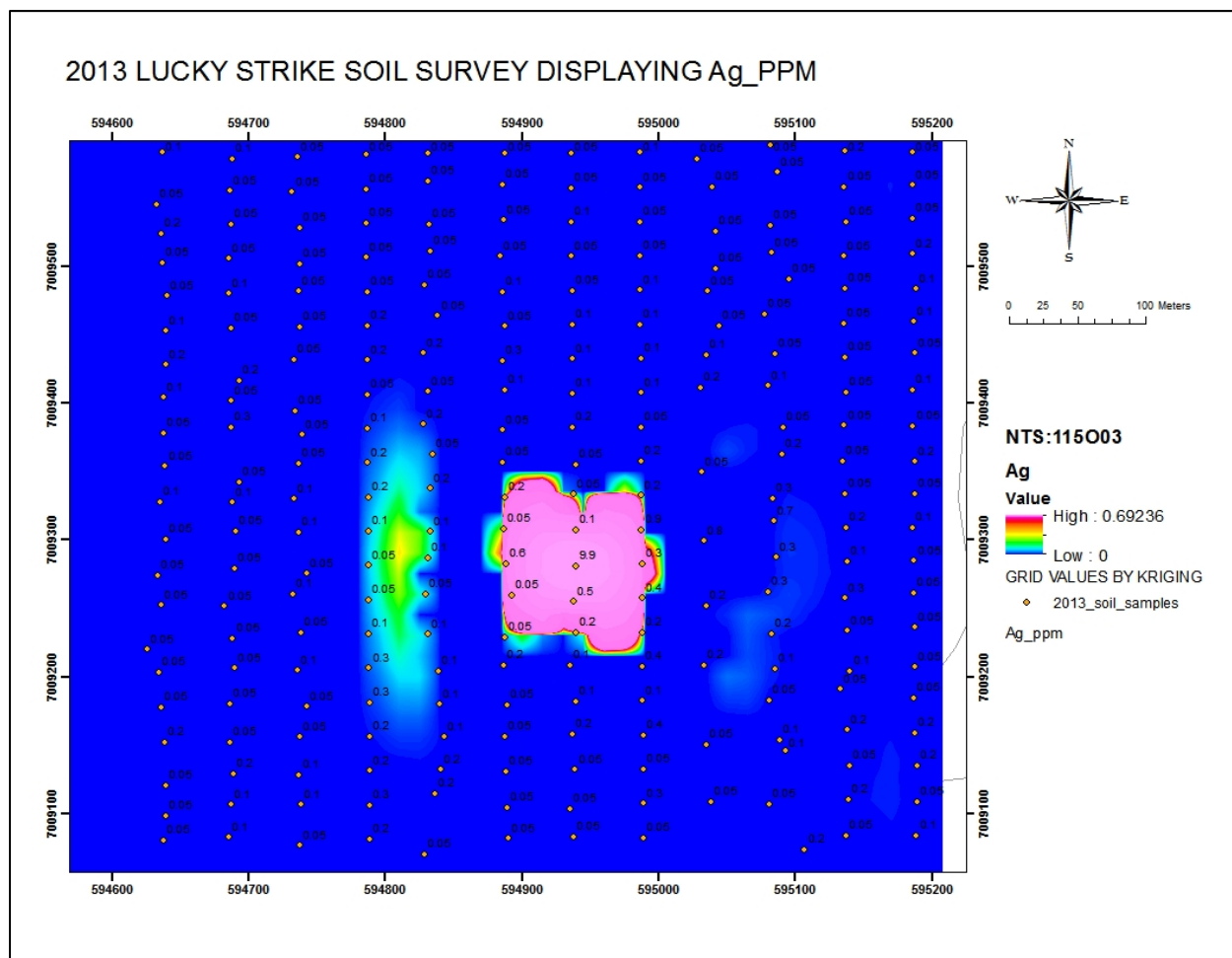
Figure 10: 2013 Soil Survey Displaying Ag ppm
