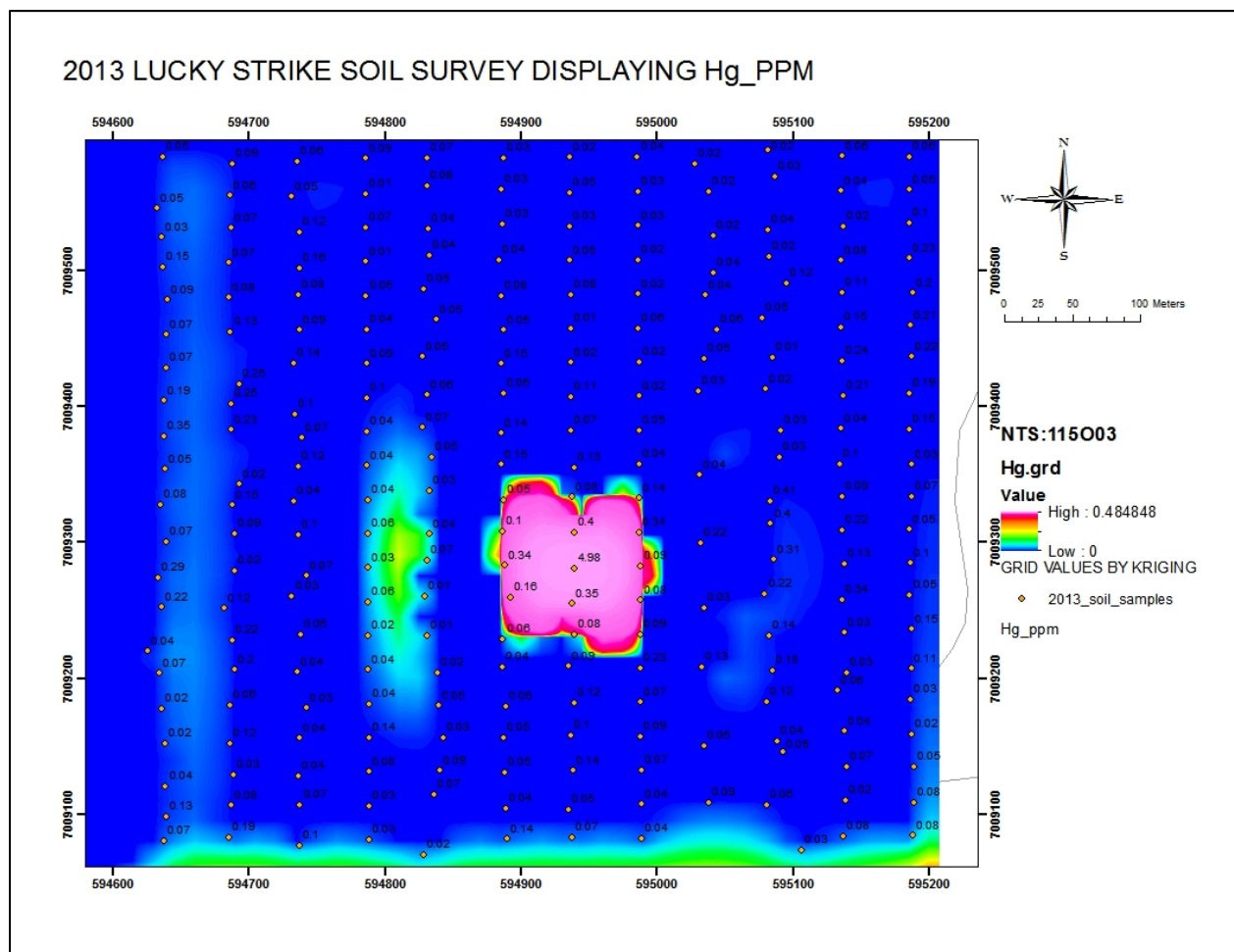
Figure 12: 2013 Soil Survey Displaying Hg ppm
