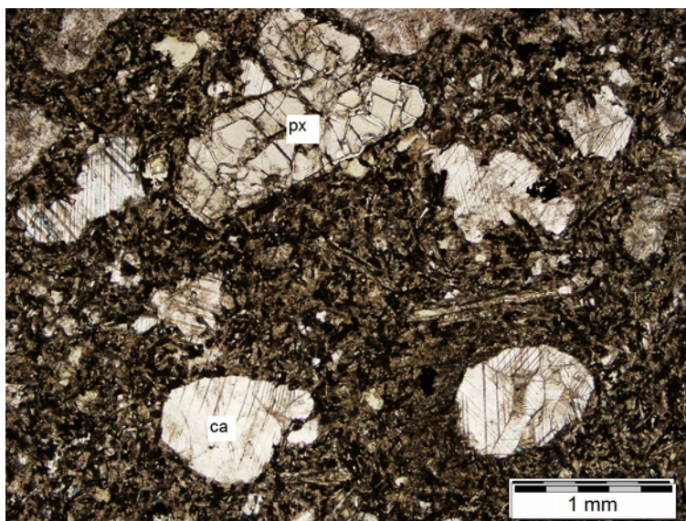
Photomicrograph 2a: Sub-rounded pseudomorphs of calcite (ca) and subhedral phenocrysts of augite? (px) are immersed within a strongly altered groundmass. Plane-polarized transmitted light.
