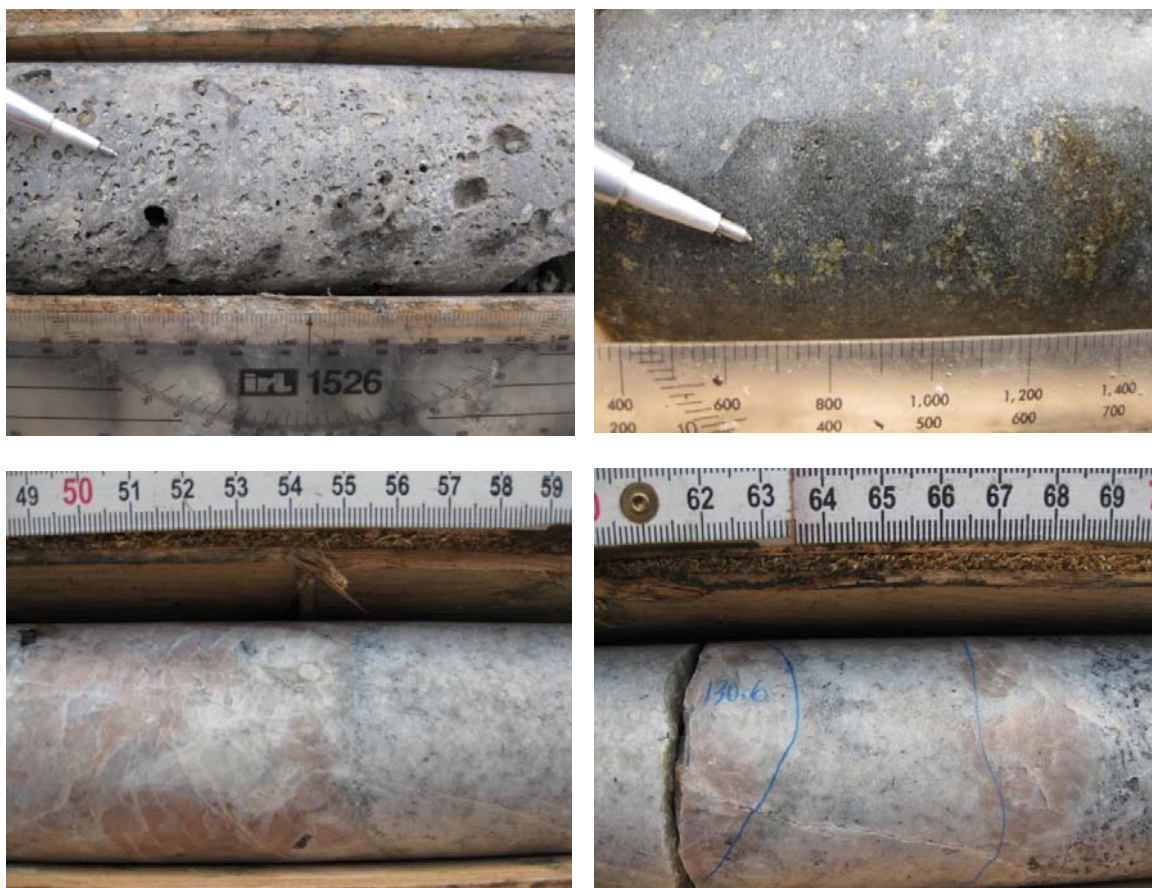
Figure 9: The top two photos show vesicular and amygdaloidal Selkirk Basalts. The bottom photos show Pegmatite dikes intruding granodiorite. The basalt was intersected in the upper part of holes KSTL-10-01 and KSTL-10-04, unconformably overlying the granodiorite.
