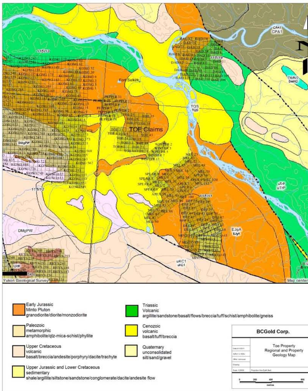
Figure 4: Toe Claims Property Geology Map. (Yukon Geological Survey, 2006)
