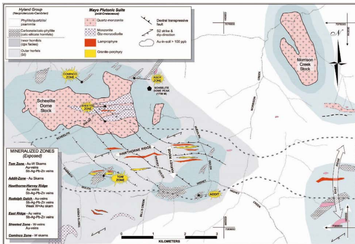
Figure 3 Generalized geological map of the Scheelite Dome area. Two main mid-Cretaceous stocks and numerous dikes intrude deformed and weakly metamorphosed Hyland Group rocks of the lower Robert Service Thrust sheet. The various intrusions in conjunction with the hornfels distribution suggest that the exposure level is co-incident with the apices of a plutonic complex. The location of significant geographic features and mineralized zones referred to in the text are highlighted. Co-ordinates are in UTM. Mineralization is concentrated in the hornfels south of the Scheelite Dome stock. Pyrrhotite envelops the stocks. Narrow lamprophyre dykes, which occupy fracture and fault zones, occur throughout the property. They are typically calcareous and commonly contain fine grained biotite and minor pyrrhotite. Fine-grained to aphanitic rhyodacite, trachyte and quartz monzonite dykes, likely related to the TPS intrusions also occur throughout the project area (Mair, 2004)
