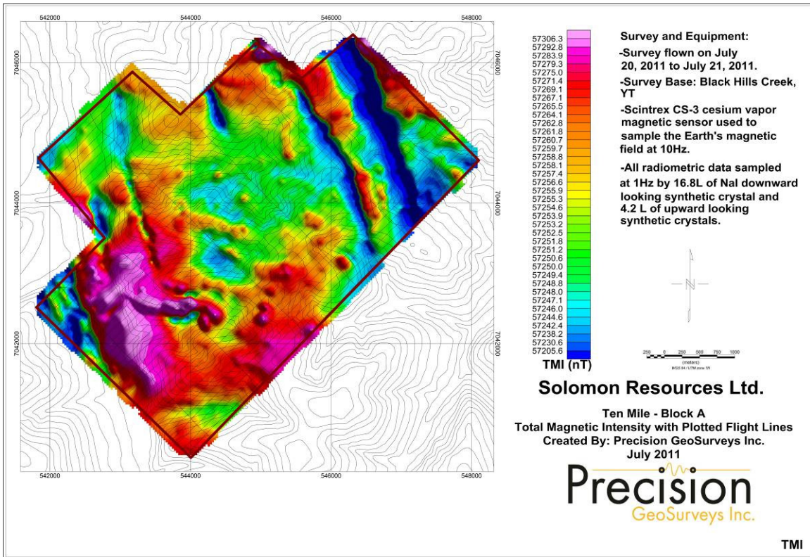
Map 2: Block A total magnetic intensity with plotted flight lines.
