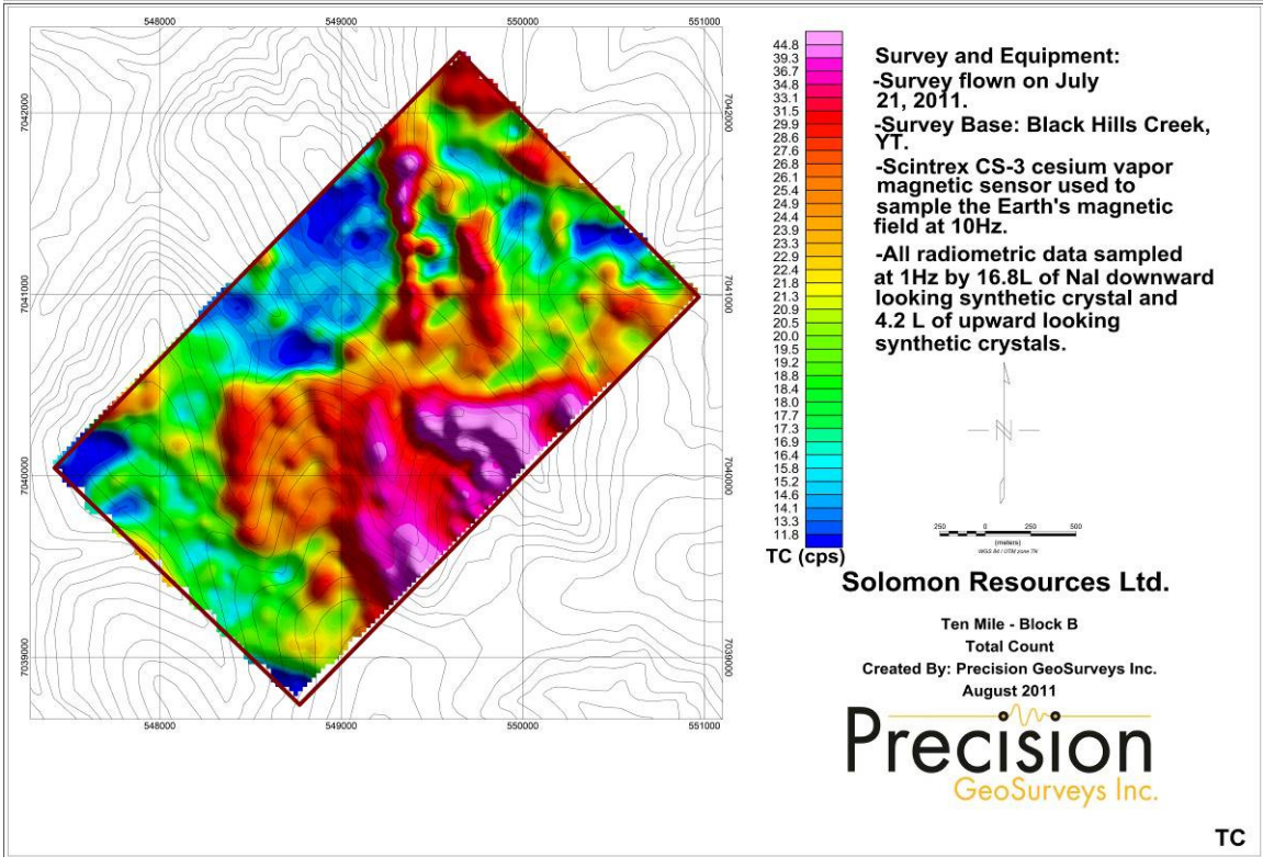
Map 7: Block B total count.
