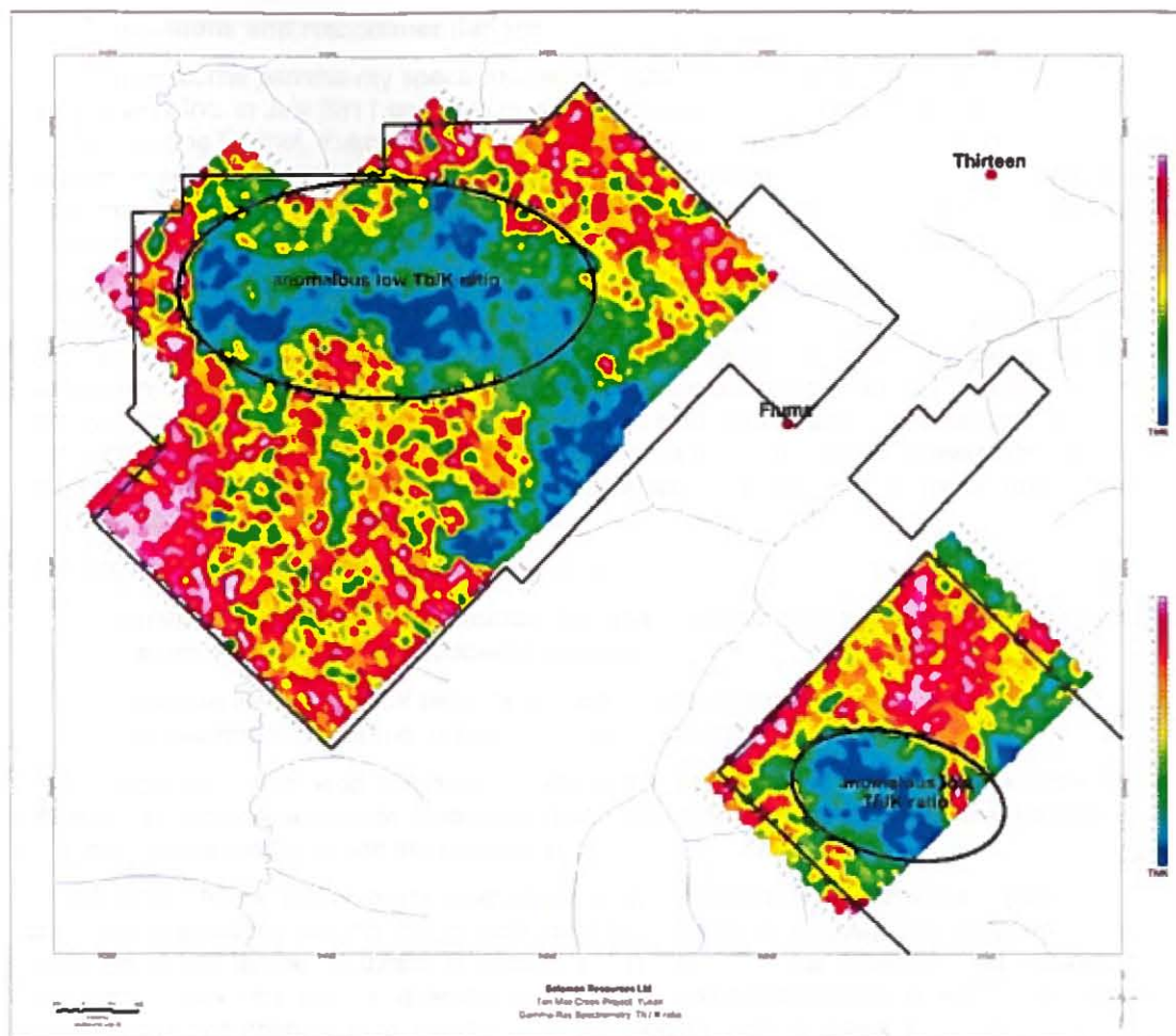
Figure 21. Th/K ratio
