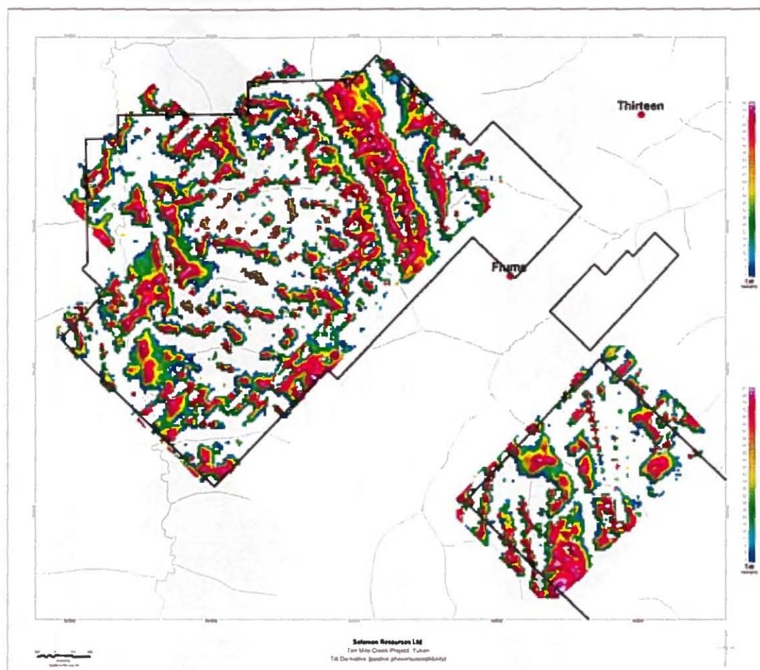
Figure 16. Tilt derivative clipped to positive phase only
