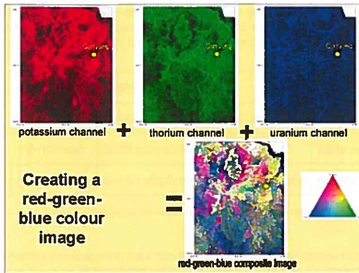
Figure 10. Ternary Image explanation
