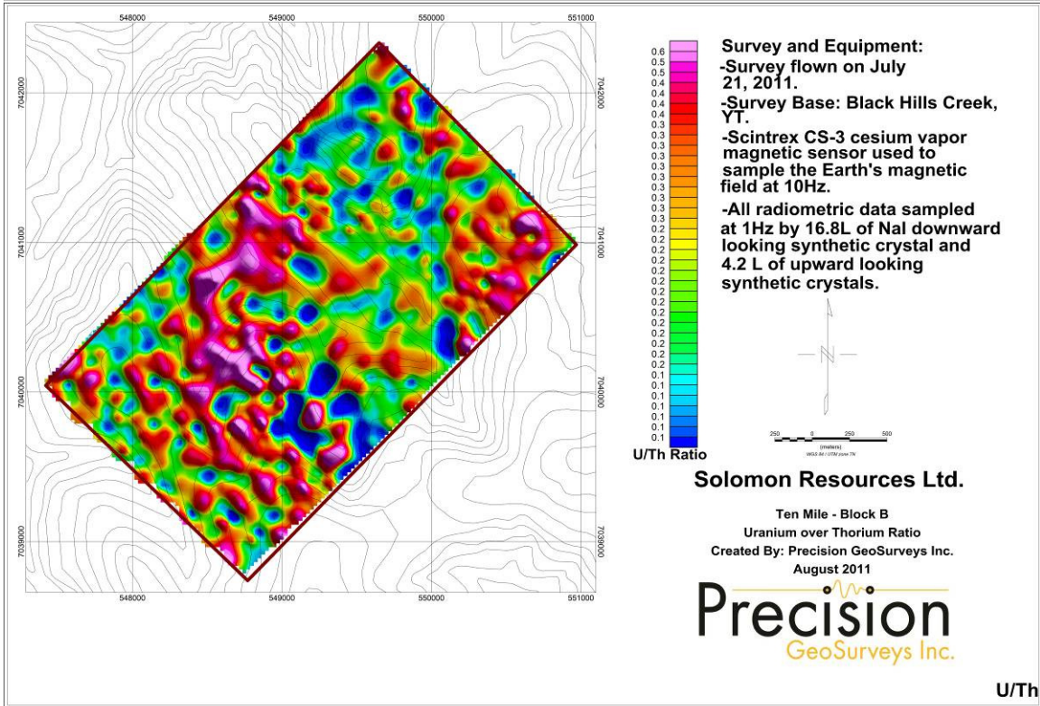
Map 10: Block B uranium over thorium ratio.
