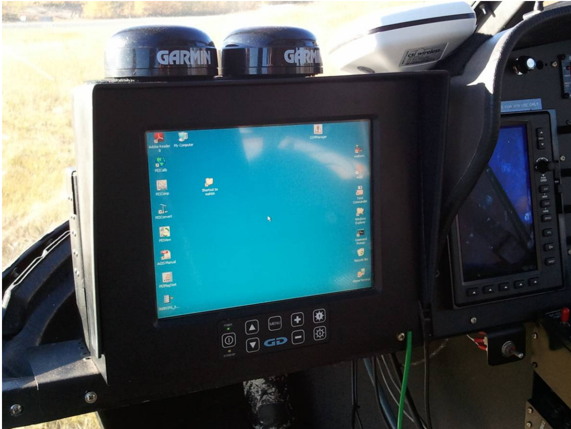
Figure 9: AGIS installed in the Eurocopter AS350 .
