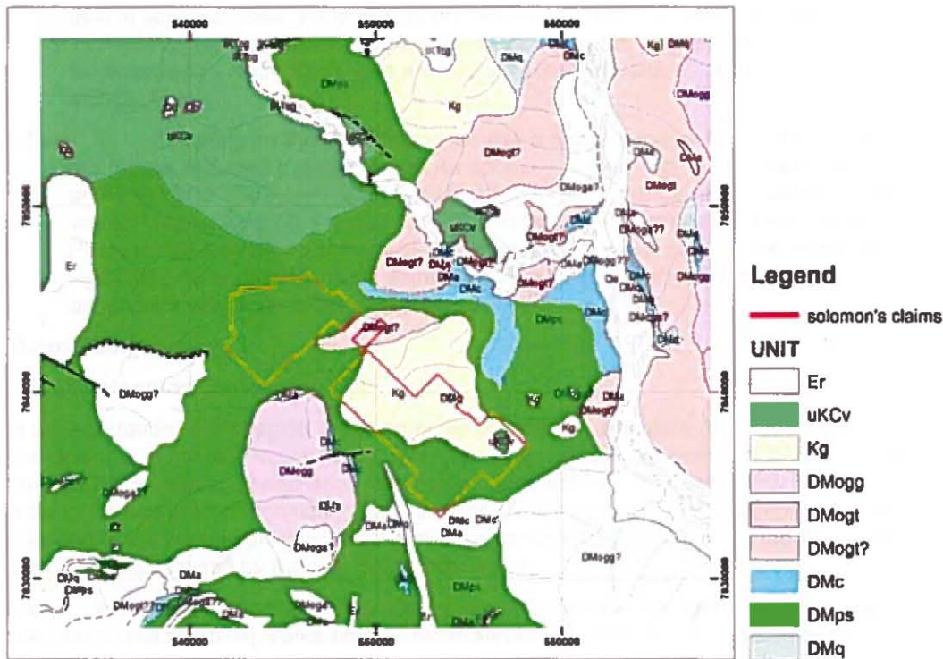
Figure 4. Regional Geology 3
