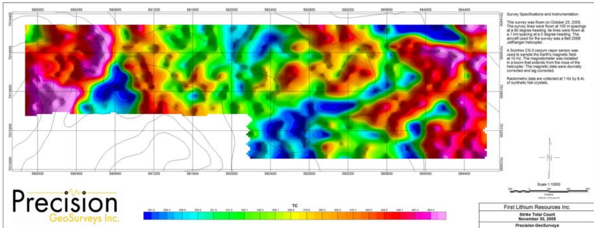
Map 2: Strike total count.
