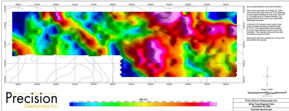
Map 1: Strike total magnetic field.
