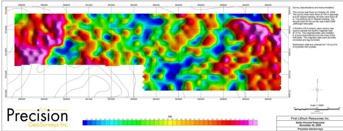
Map 3: Strike percent potassium
