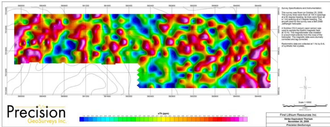
Figure 5: Strike equivalent thorium
