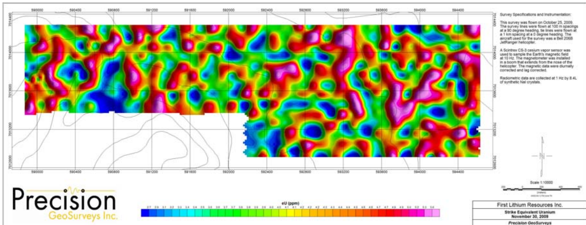
Map 4: Strike equivalent uranium
