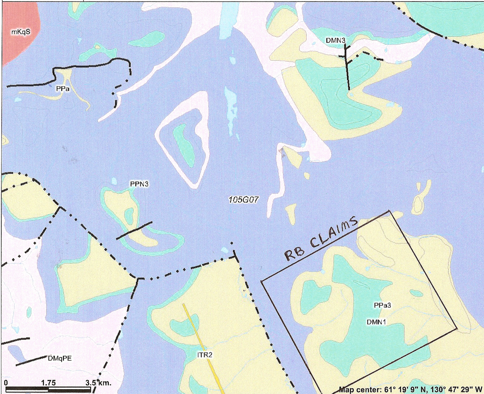
Figure 3 Regional Geology
