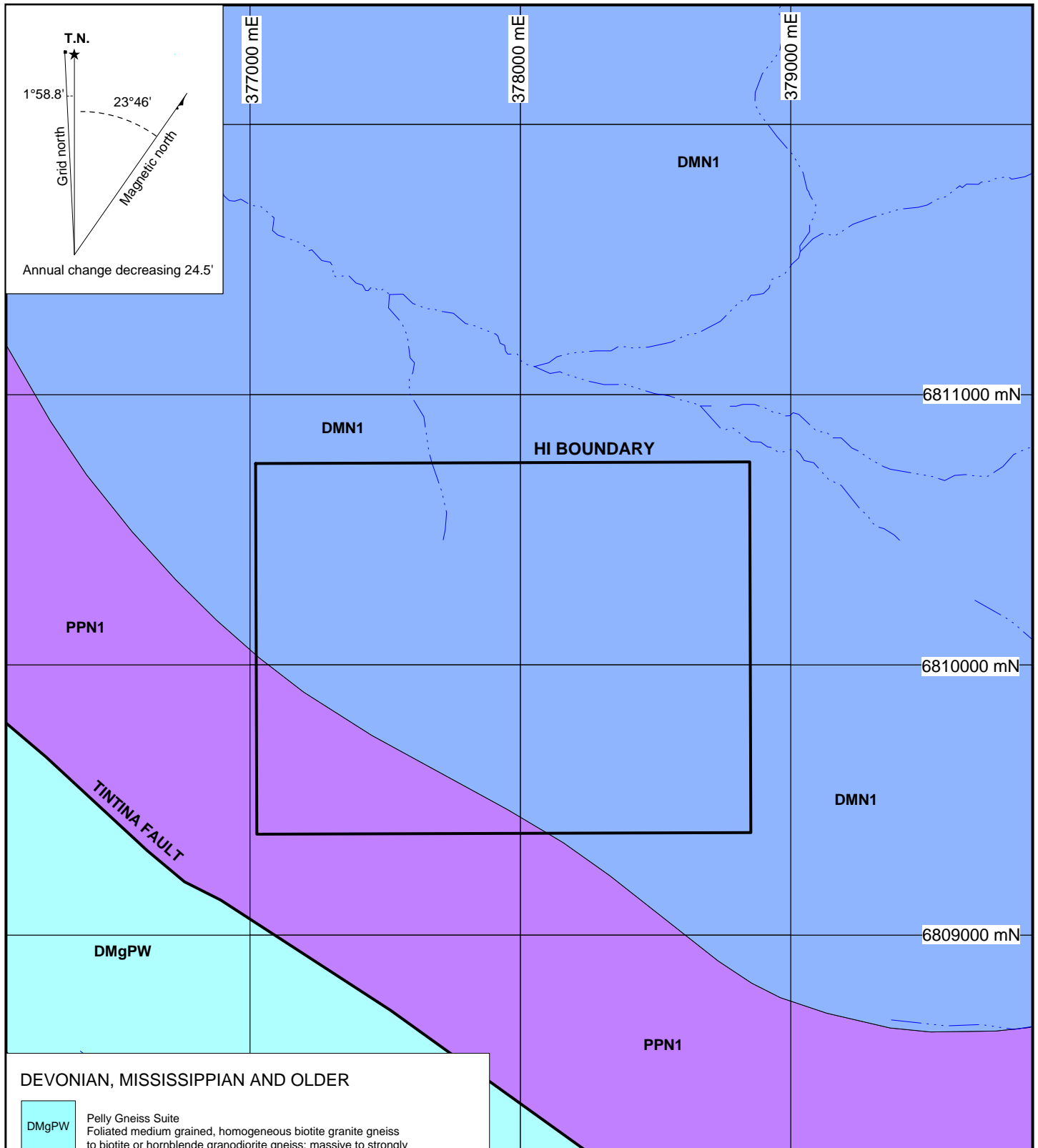
FIGURE 4 ARCHER, CATHRO & ASSOCIATES (1981) LIMITED REGIONAL GEOLOGY HI PROPERTY
