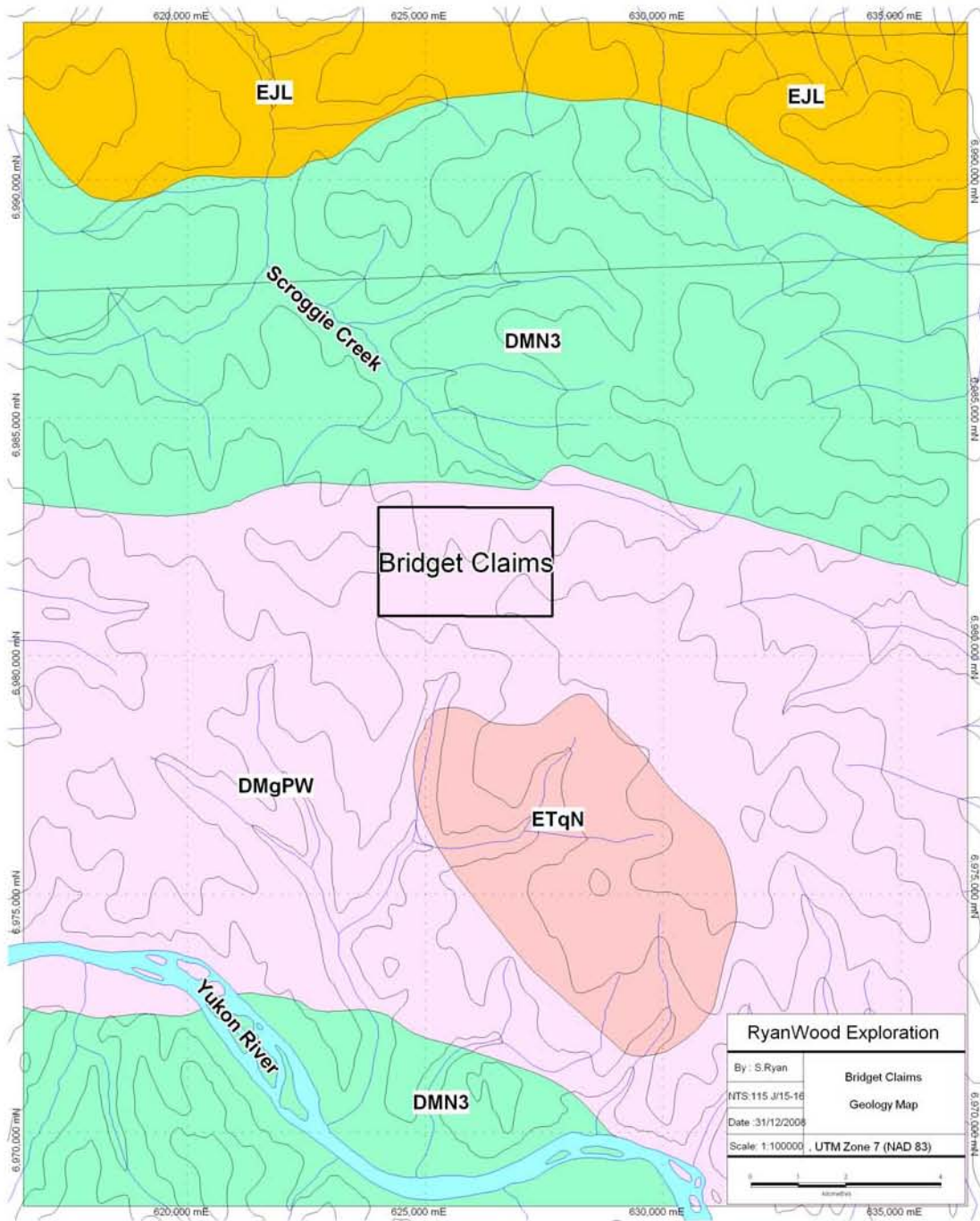
Yukon Geology Map
