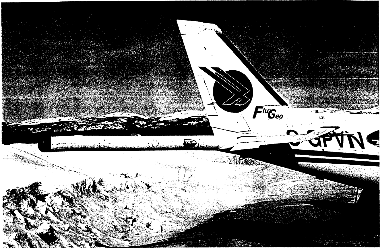
Figure 9: Tail stinger of the aircraft with CS-3 Mag sensor
