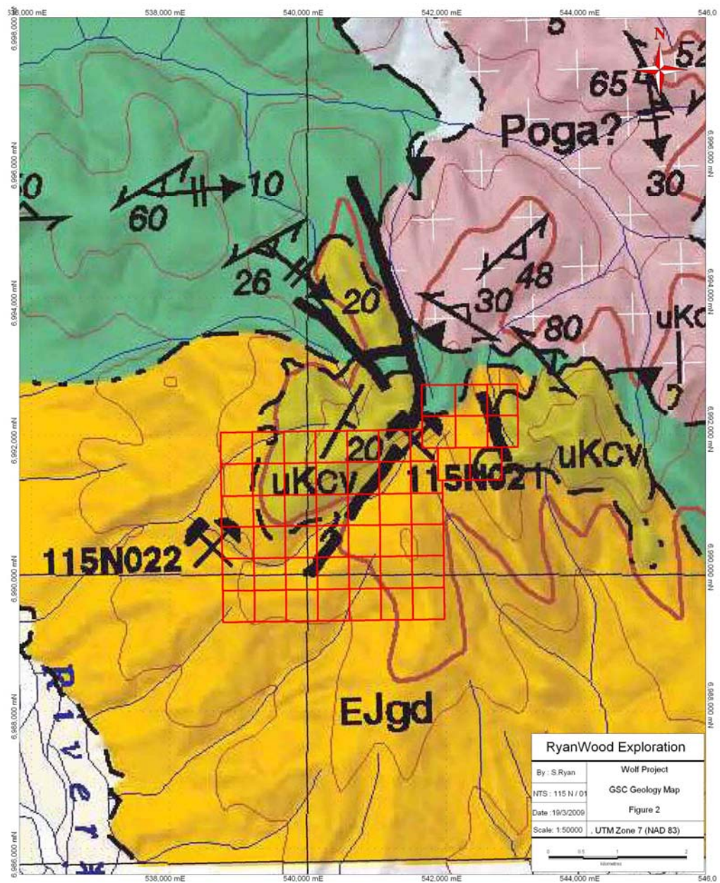
GSC Geology Map
