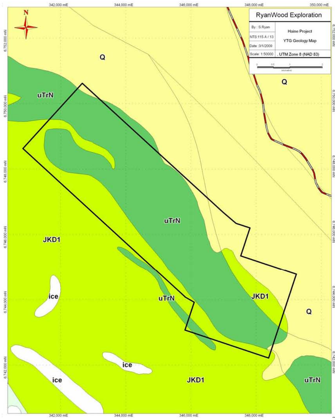
YTG Geology Map
