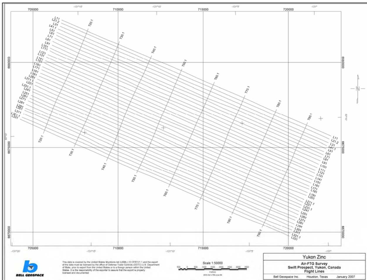
Figure A 2. Survey actual flight lines.
