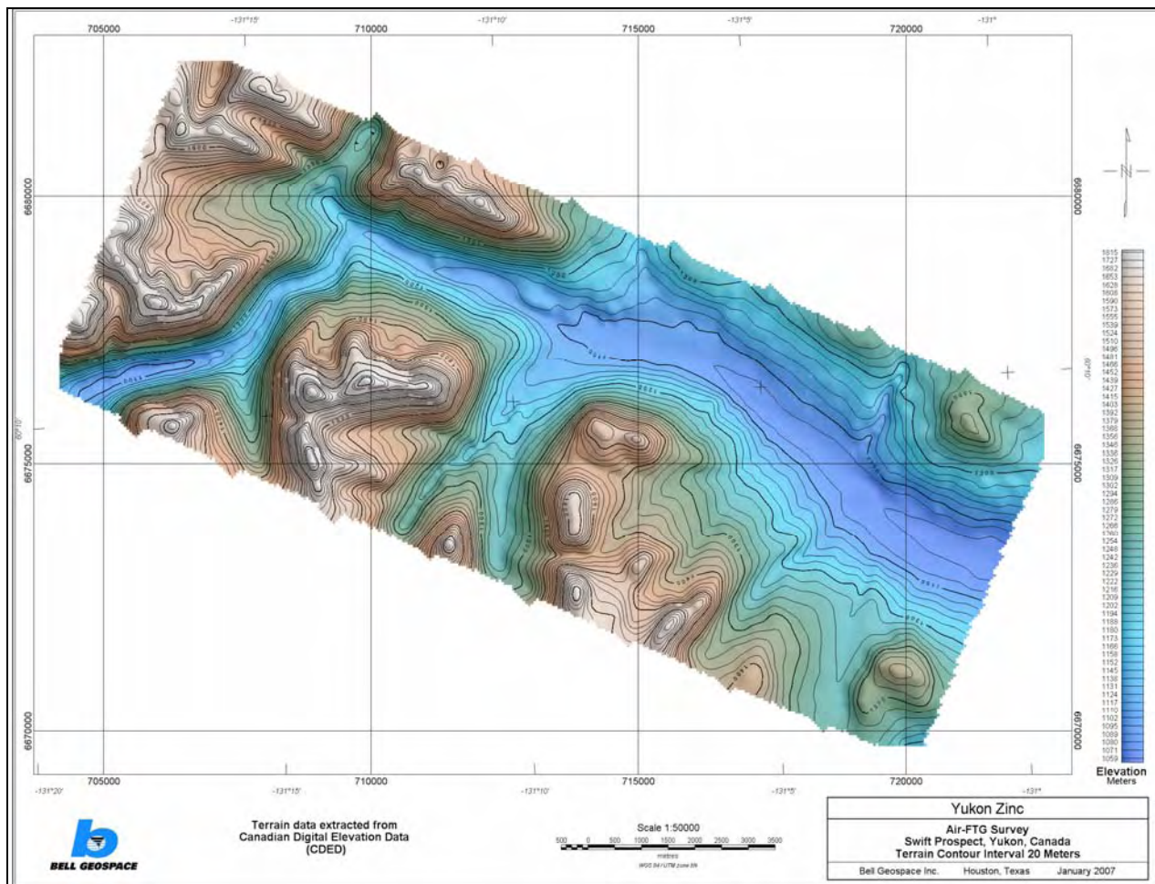
Figure A 3. Digital terrain model compiled from CDED Terrain data.
