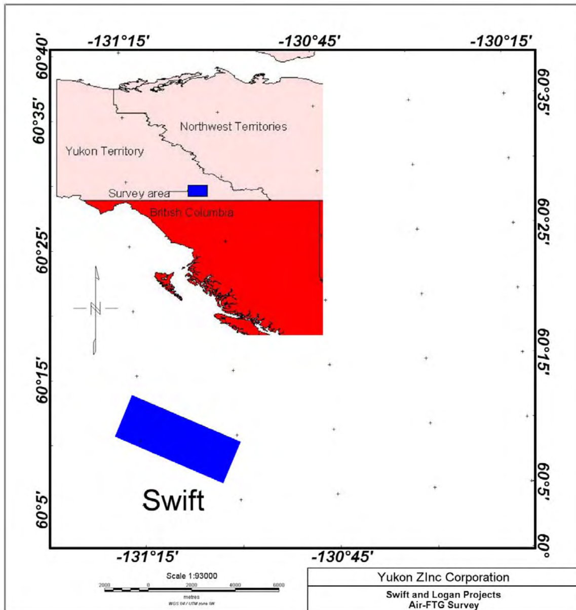
Figure A 1. Swift prospect survey location shown in a blue box.
