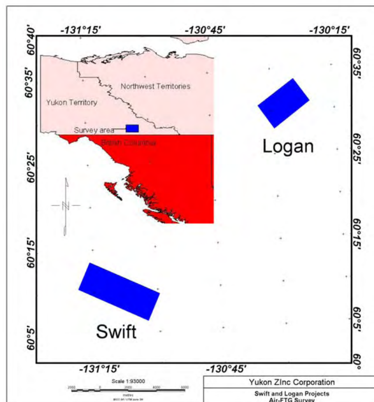
Figure 1. This map indicates the position of the individual survey blocks, along with an insert that shows the general location of the survey area in Yukon Territory.
