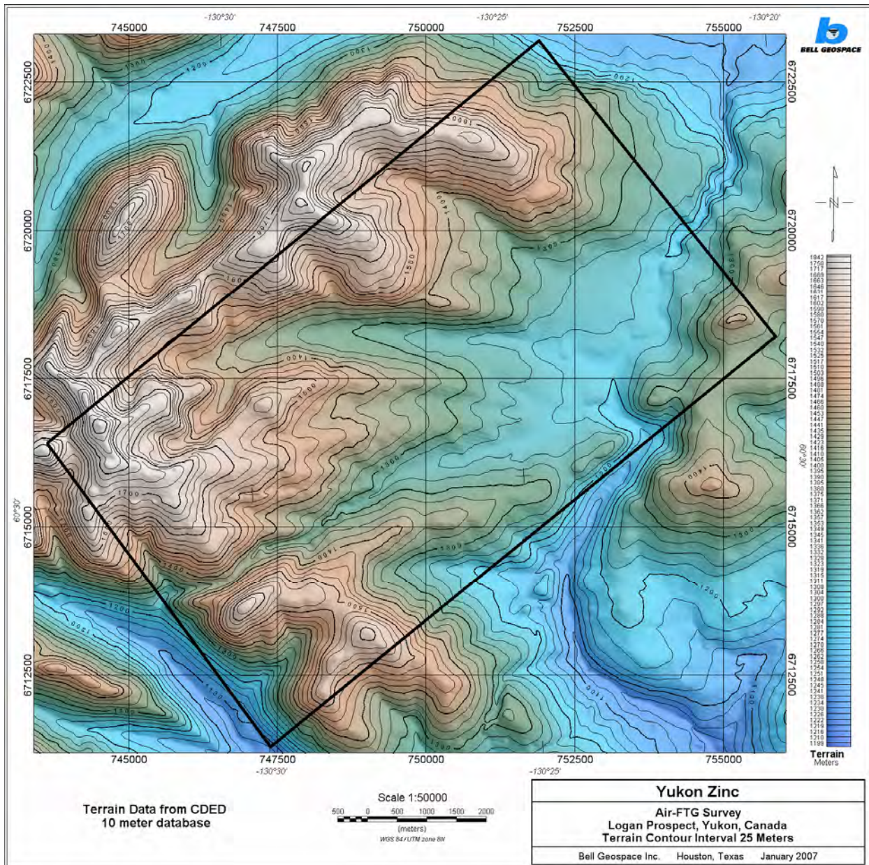
Figure B 3. Digital terrain model compiled from CDED Terrain data. The black box inside the DEM marks the survey area boundary
