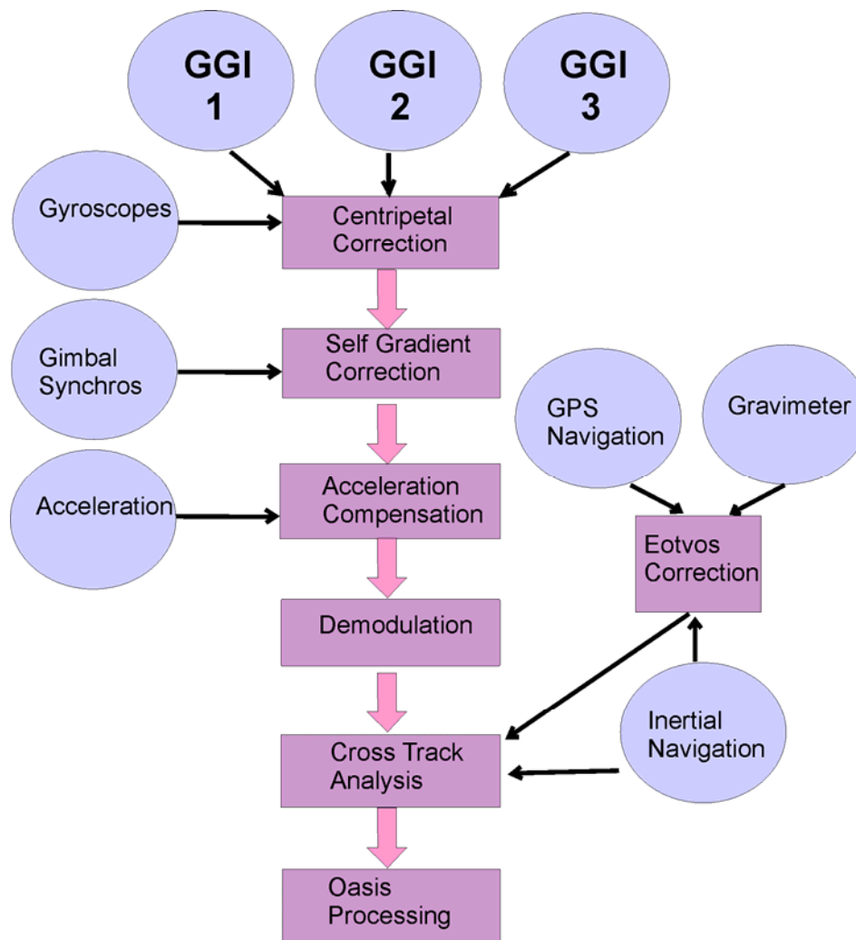
Figure 2.1: A schematic diagram showing different stages of FTG Data Processing
