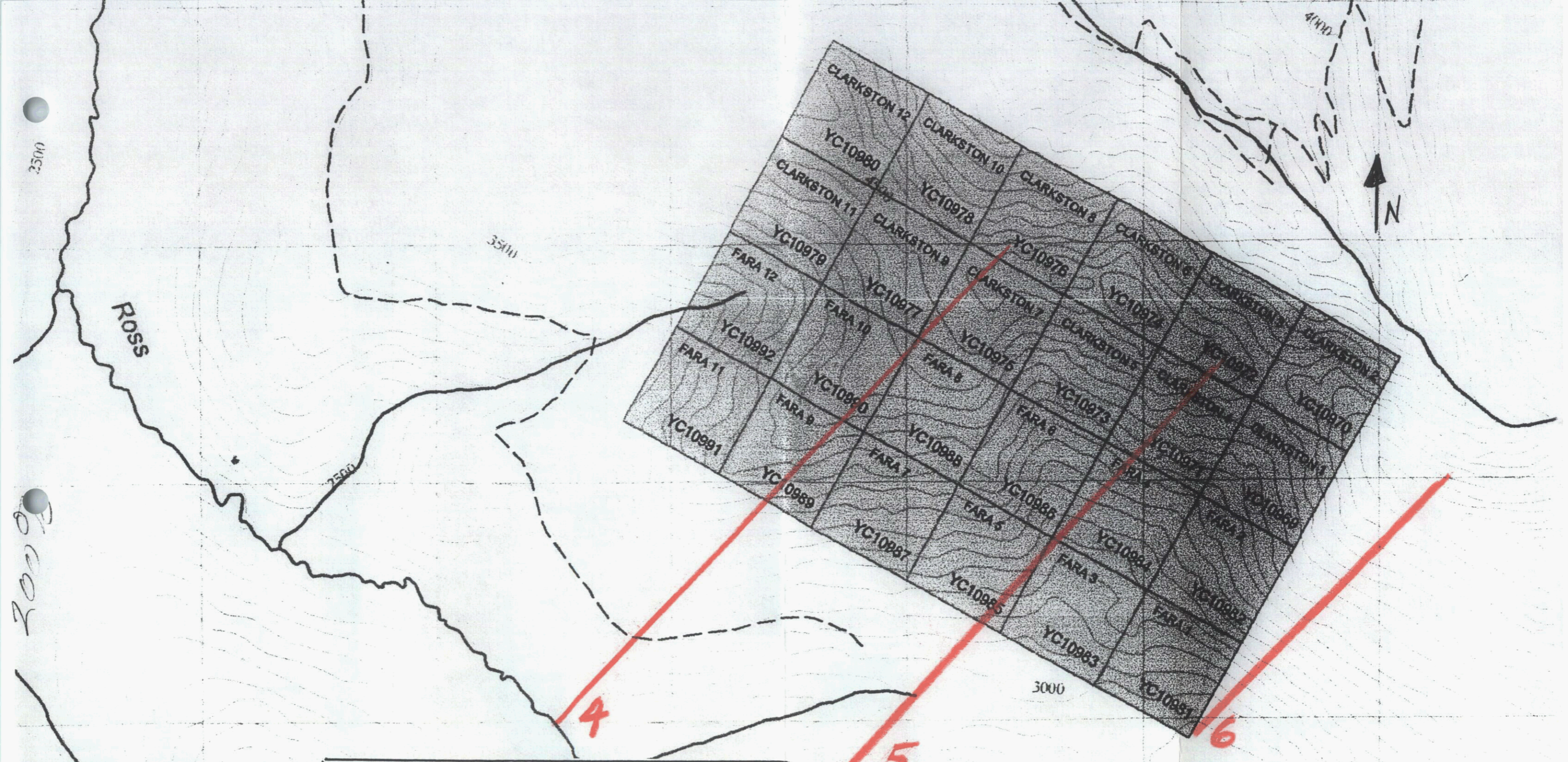
FIGURE # 4B (WEST) SOIL SAMPLE LOCATION MAYO MINING DISTRICT NTS. 105 M 13 — SOIL SAMPLES (PAST) DATE 20 NOV. 2003 DRAWN BY JP ROSS SCALE 1:15,000
