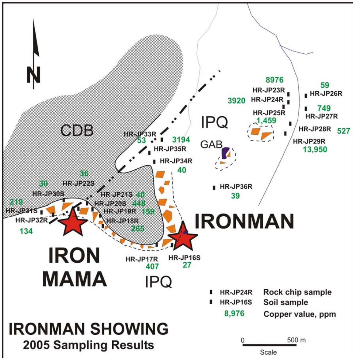
Figure 5 - Results of 2005 sampling, Ironman showing area.
