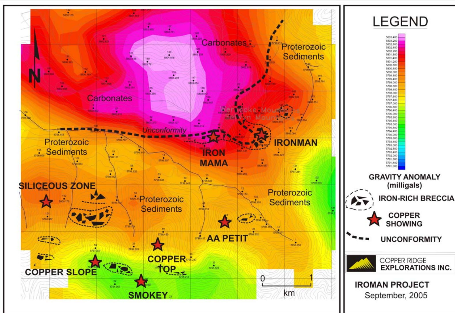
Figure 6 - Ironman Gravity Survey - Bouguer Anomaly Map.
