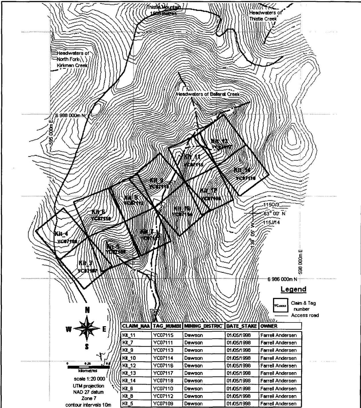
Figure B: Map showing the KIT 3-14 claims on NTS mapsheets 115O/3 & 115J/14
