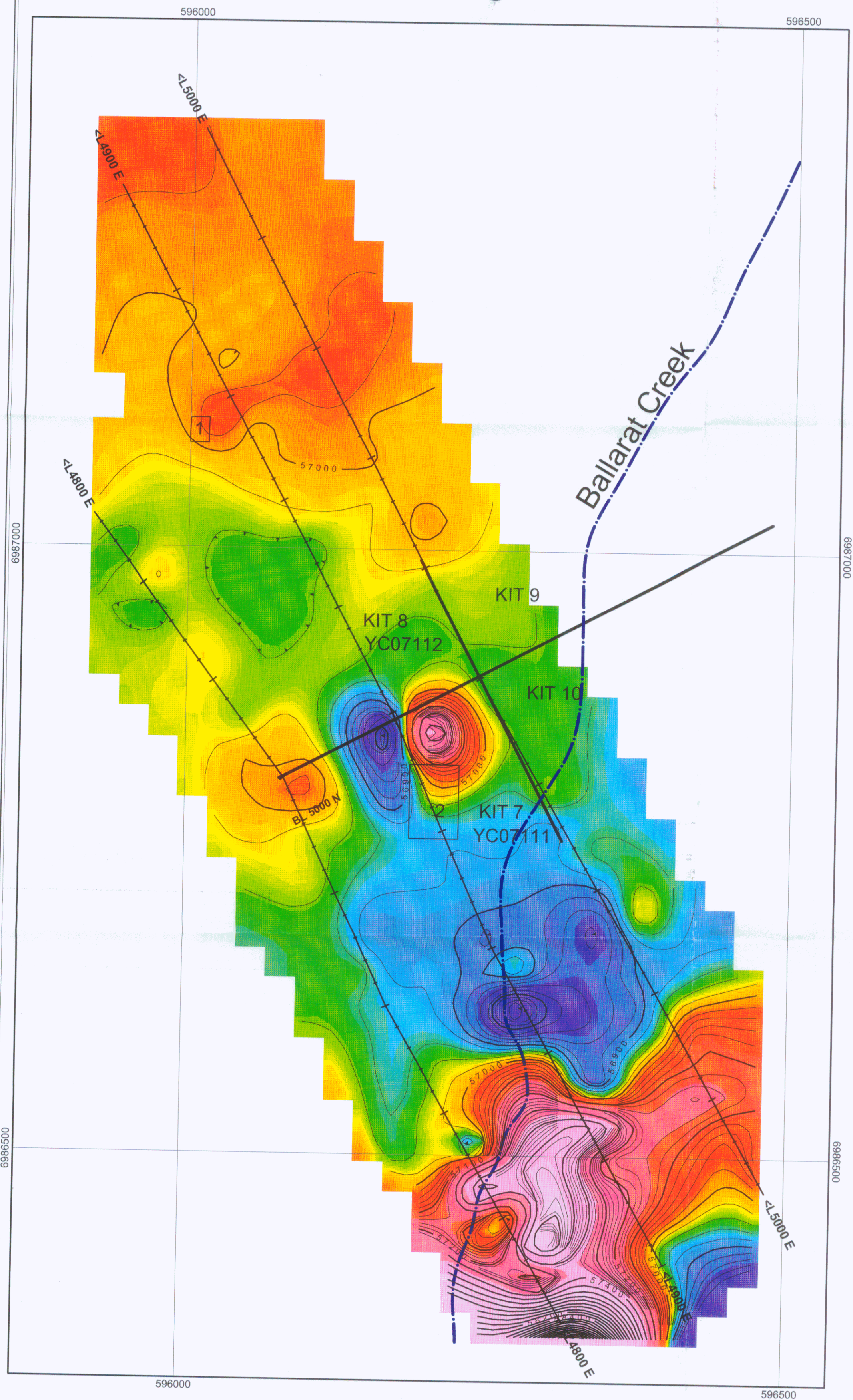
Figure D: Total Field Magnetics for the KIT 7 & KIT 8 Claims
