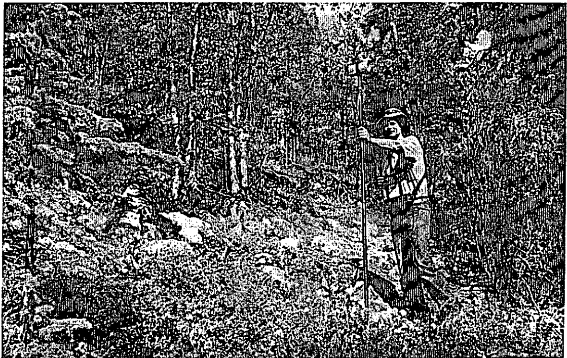
Photo 4: Ground magnetometer survey on the KIT 7 claim
