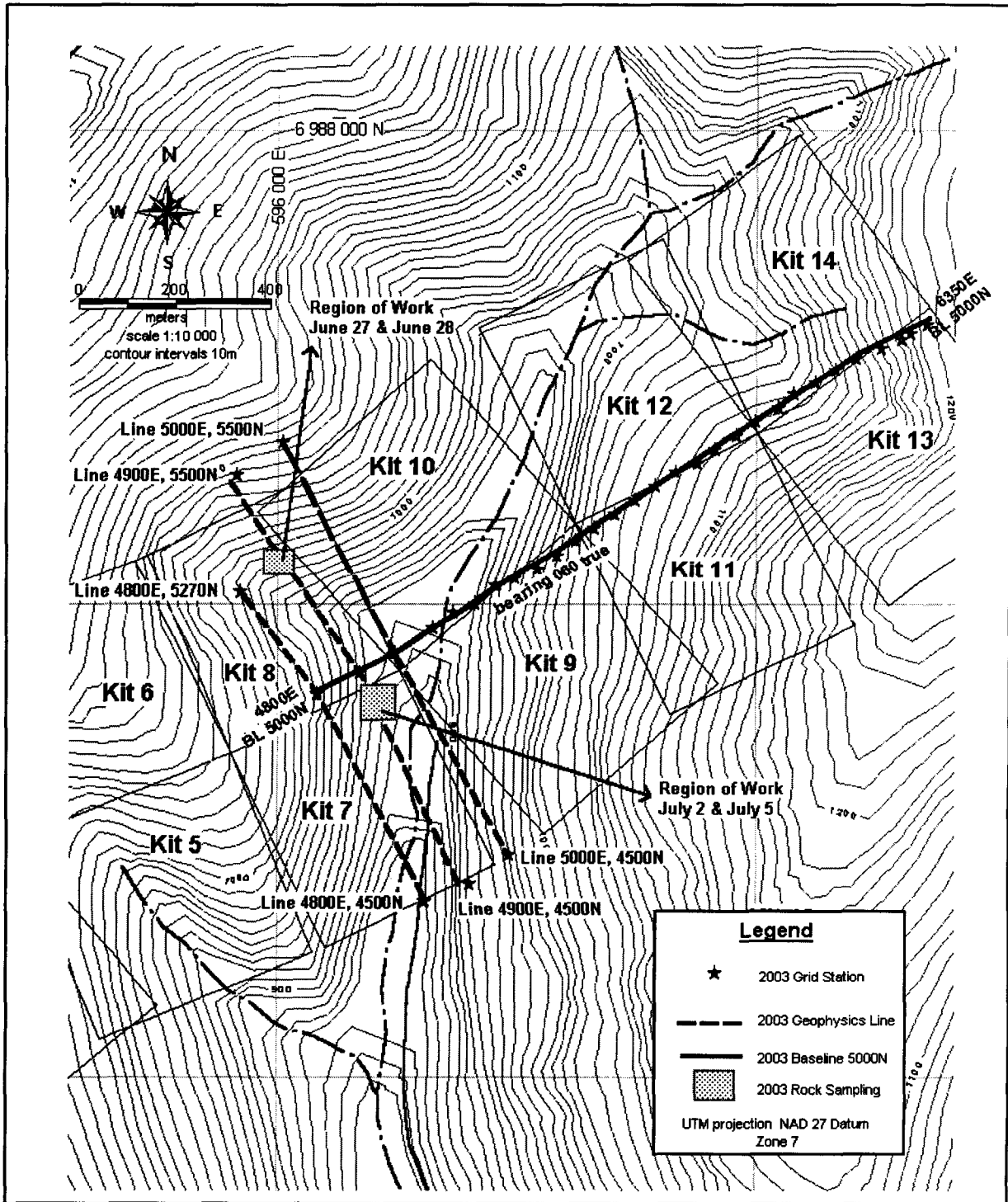
Figure C: Map showing work done for the 2003 work program. Grid lines surveyed by magnetometer appear as black dashes. The solid black line is the established baseline on the east half of the property. Hand-held GPS defined stations are shown as stars. Regions prospected and sampled in 2003 are outlined as patterned rectangles.
