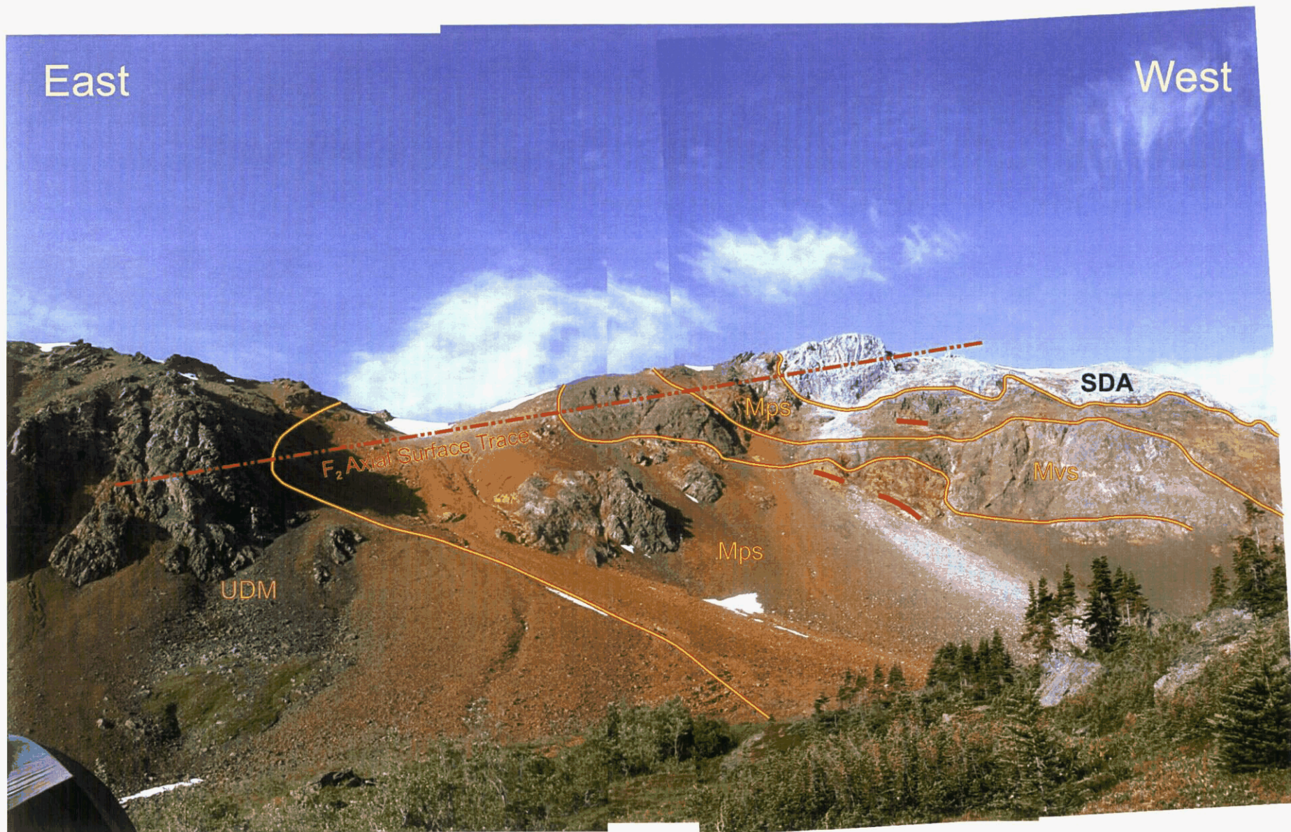
Plate 1 - Composite view, looking south, at the well exposed outcrops of the MM claims with the major map units delineated. The axial surface trace of the large-scale, recumbent F_2 fold hinge skims the ridgeline. Areas of significant mineralization (semi-massive to massive sulphides) are delineated in red. The field of view is approximately 750 meters east to west. Man, that was a nice day!
