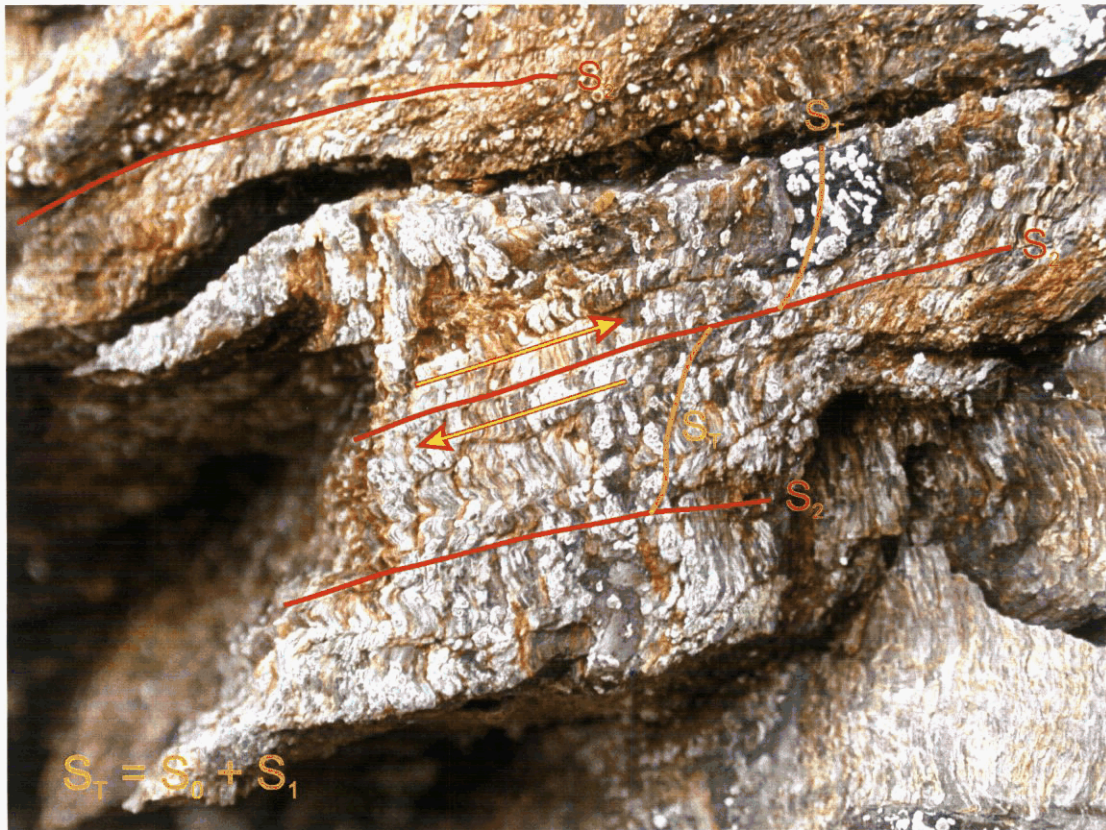
Plate 5 - Typical structural style of an F_2 fold hinge. S_{T1} is being folded by a recumbent F_2 fold and shearing is taking place along the well developed S_2 cleavage.
