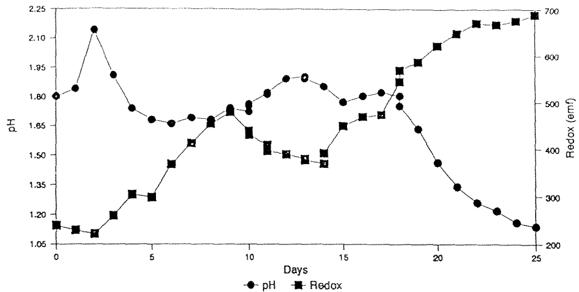
FIGURE 5-1 CONCENTRATE BATCH BIOLEACH TEST pH and Redox vs Time
