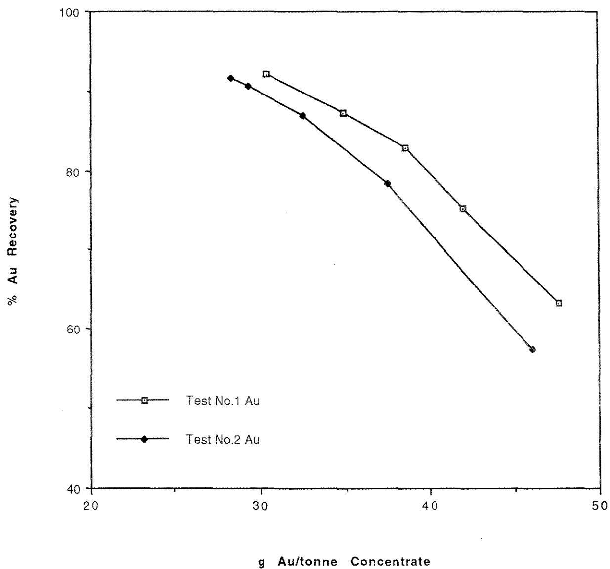
FIGURE 4-2 SKUKUM CREEK RAINBOW FLOTATION TESTS % Au Recovery vs g Au/tonne Concentrate
