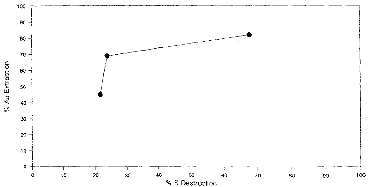
FIGURE 5-6 CONCENTRATE BATCH BIOLEACH TEST Au Extraction vs S Destruction
