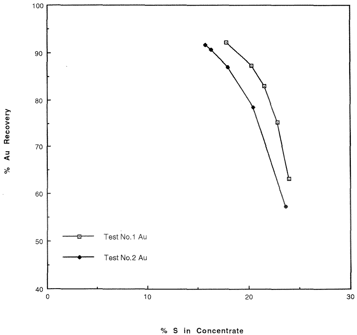
FIGURE 4-3A SKUKUM CREEK RAINBOW FLOTATION TESTS % Au Recovery vs % S in Concentrate
