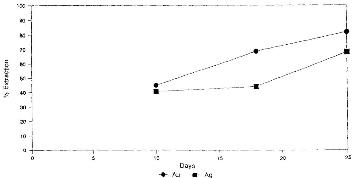
FIGURE 5-4 CONCENTRATE BATCHS BIOLEACH TEST Au and Ag Extraction vs Time
