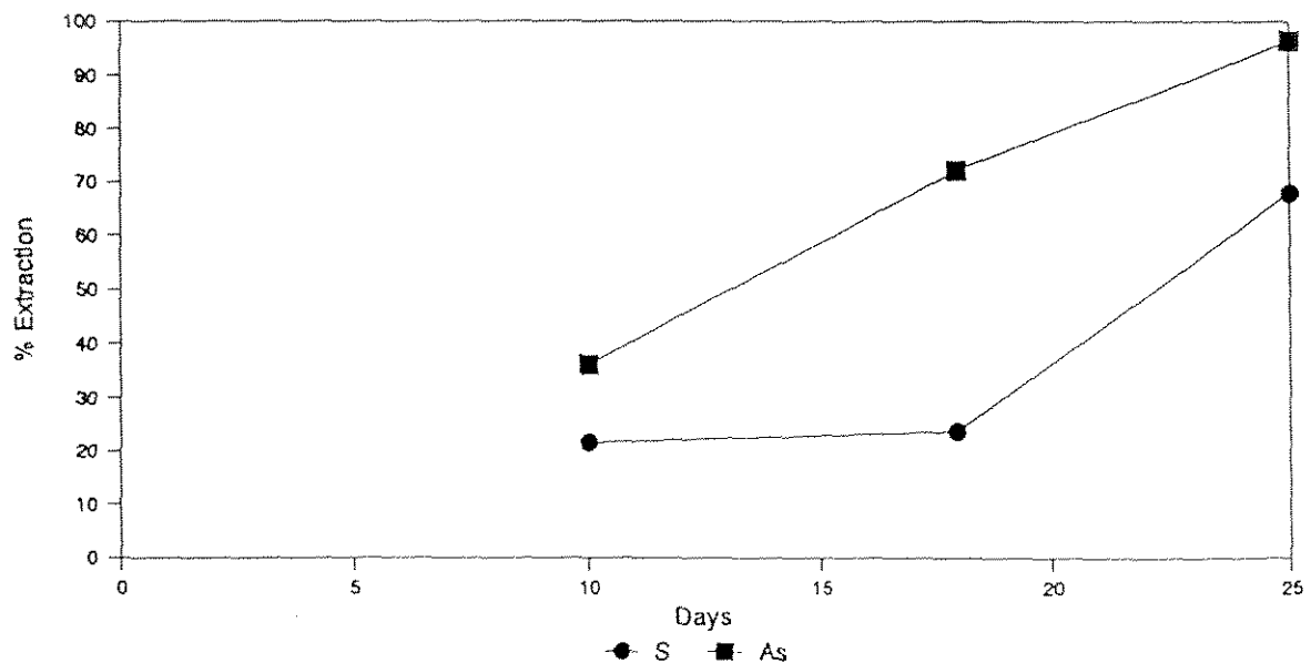
FIGURE 5-2 CONCENTRATE BATCH BIOLEACH TEST S and As Extraction vs Time
