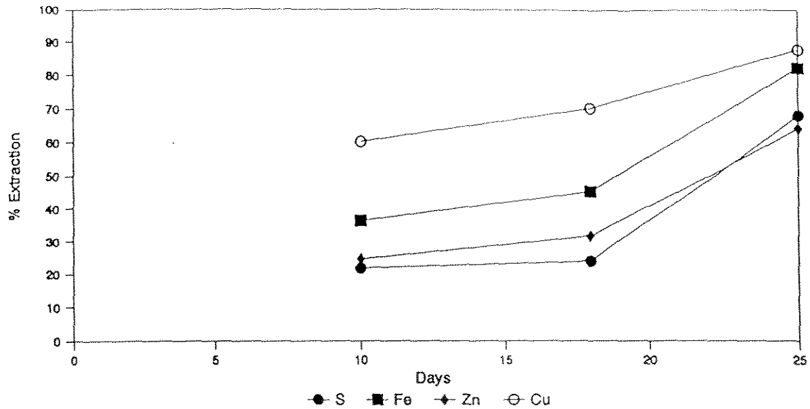
FIGURE 5-3 CONCENTRATE BATCH BIOLEACH TEST S, Fe, Zn and Cu Extraction vs Time
