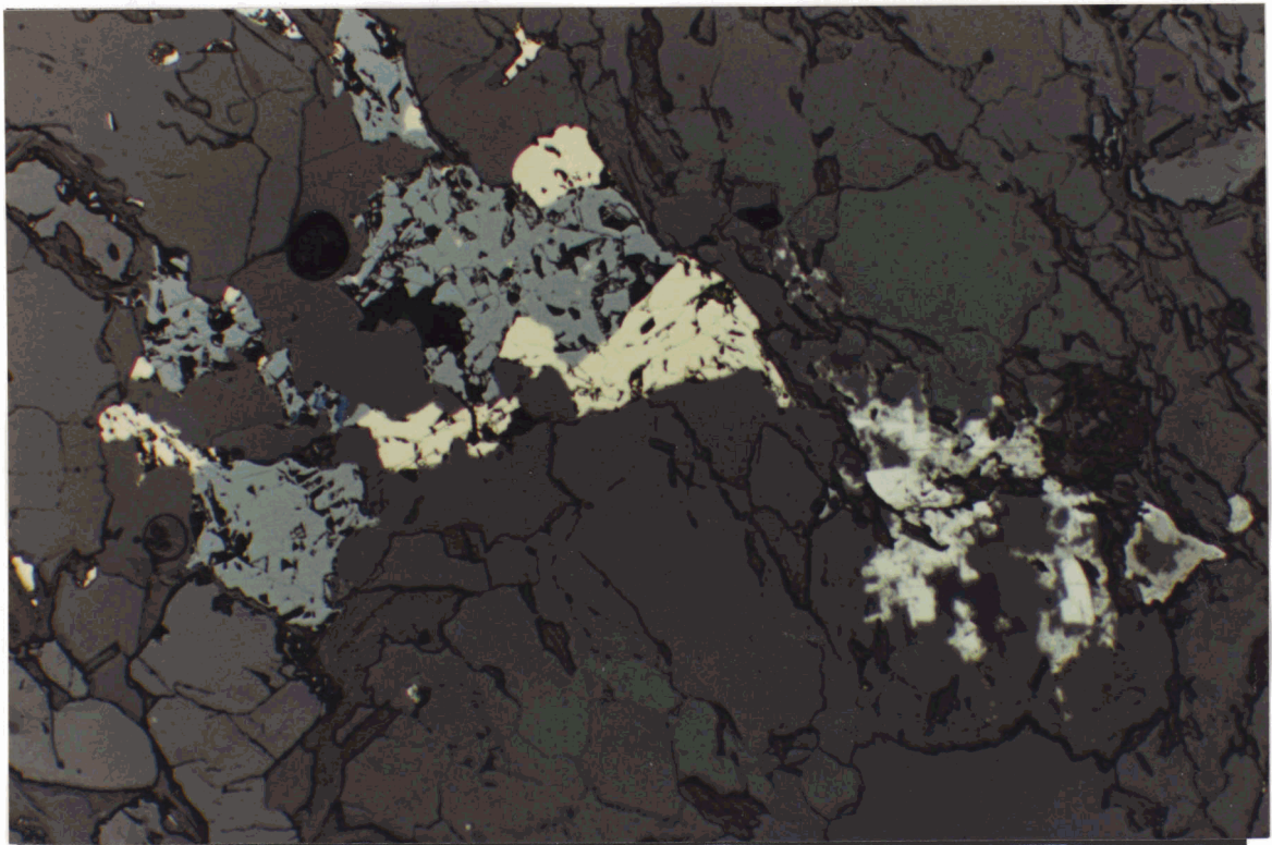
Sample A: Reflected light views (plane polarized) showing sphalerite (light grey) pyrite (white) and chalcopyrite (creamy) grains. Same field of view as previous (above, 3 mm wide) and enlarged (below, 1.3 mm wide) showing composite sphalerite-chalcopyrite-minor covellite grains and pyrite after pyrrhotite (dark grey high relief grains are garnet).
