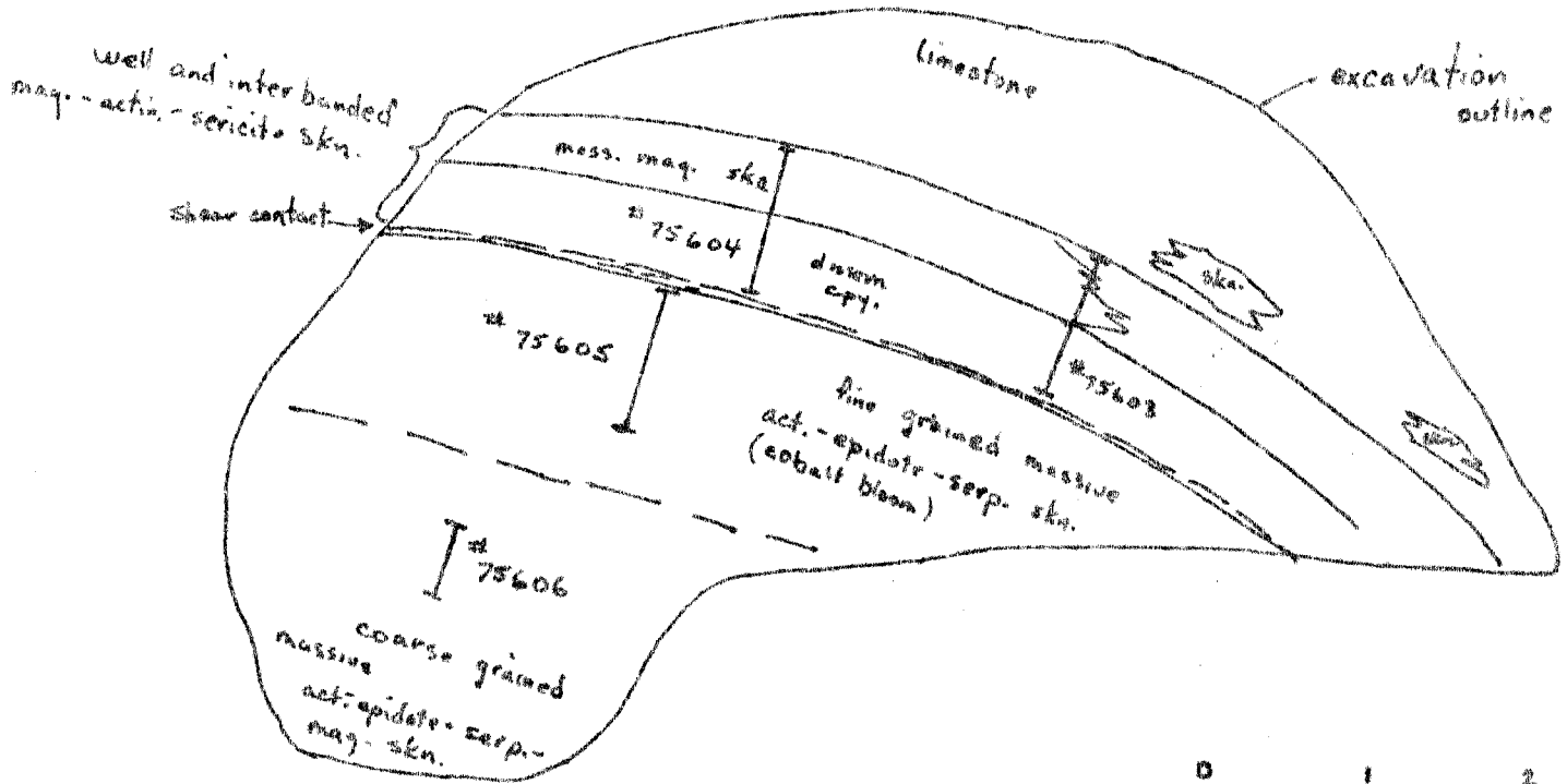
X-SECTION
