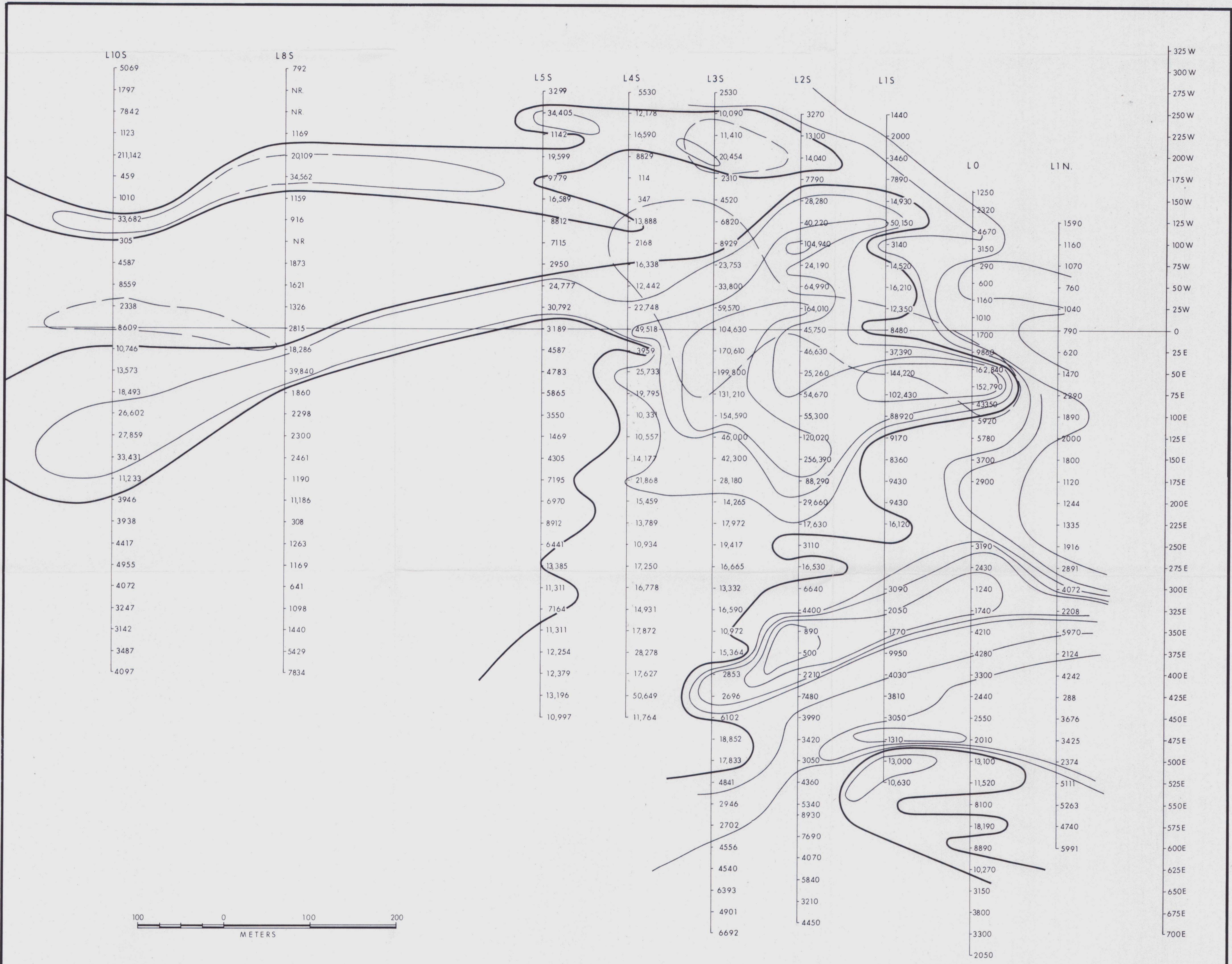
Fig. No. 8 AQUITAINE COMPANY OF CANADA Ltd. INDUCED POLARIZATION SURVEY APPARENT RESISTIVITY PLAN BONNET LAKE, YUKON (VALUES IN OHM · M) POLE-DIPOLE ARRAY G=25m. N=4
