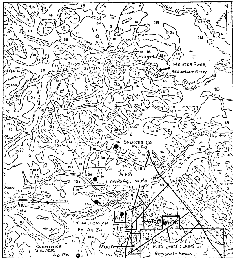
FIGURE 3. Regional geology of Rancharia area, Y.T., Portion of G.S.C. Map 10 - 1960 (Wolf Lake). Scale: 1 in = 4 miles.
