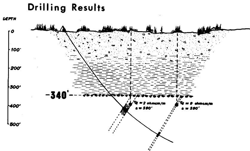
Figure 7.—Turam traverse over deeply buried conductors in the Timmins area.
