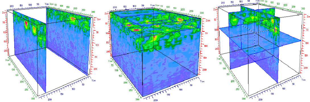
Fig. 2 Three-dimensional visualization
