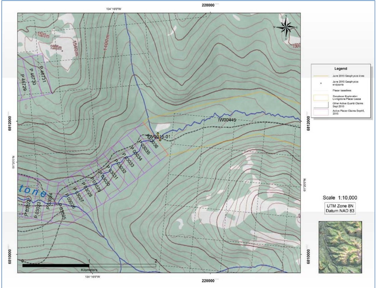
Figure 2 – Location of Geophysical resistivity line LC A (LIV2015-01) conducted by Kryotek on lower Livingstone Creek, on Prospecting Lease IW00445.
