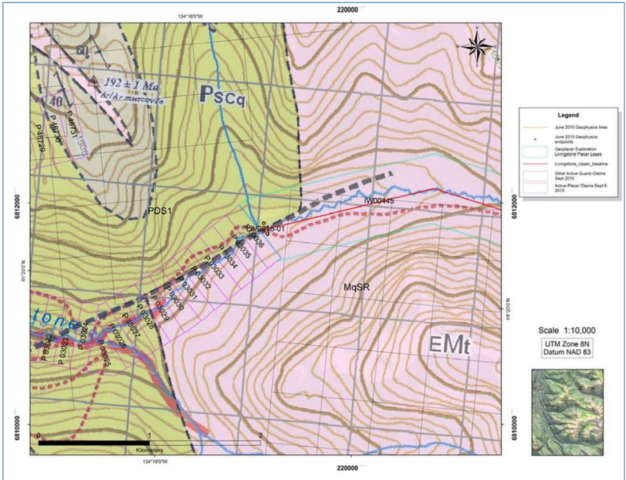
Figure 3 – Bedrock Geology of Livingstone Creek at the location of the geophysical resistivity line LC A (LIV2015-01) on Prospecting Lease IW00445. After Colpron, M., 2005. Geological map of Livingstone Creek area (NTS 105E/8), Yukon (1:50 000 scale). Yukon Geological Survey, Open File 2005-9.
