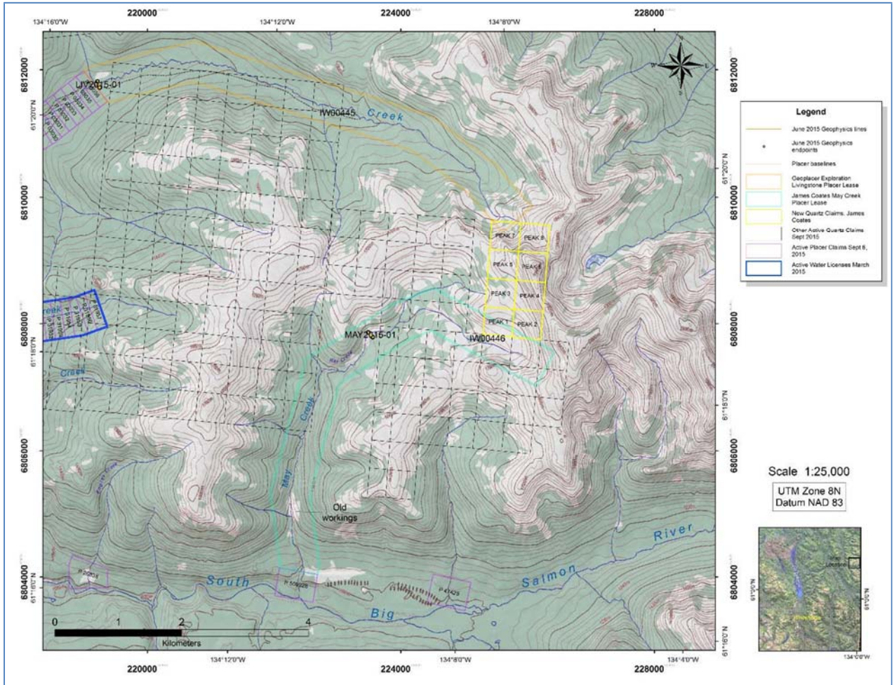
Figure 1 – Location of Geophysical lines conducted by Kryotek in Livingstone region in June, 2015.
