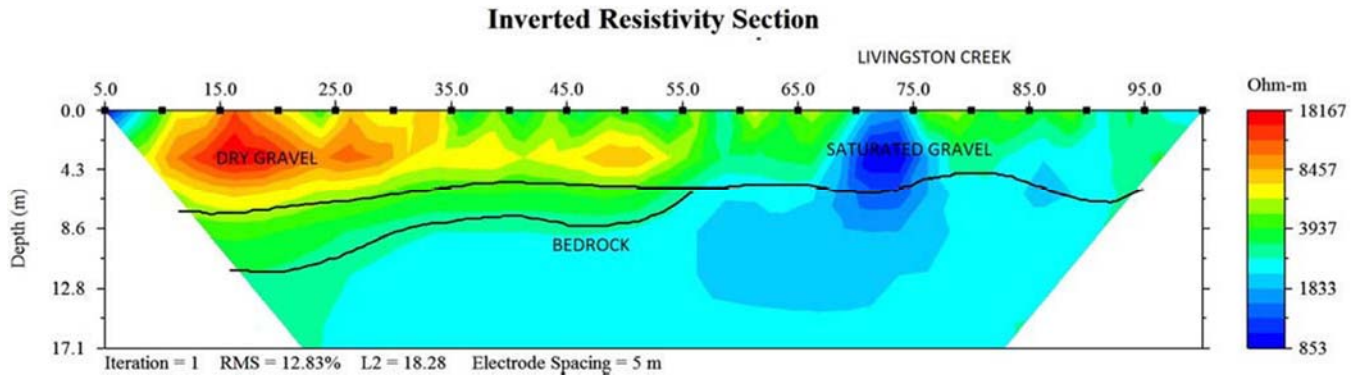
Figure 4 - Geophysics line LC A on prospecting lease IW00445 on Livingstone Creek. The location of this survey is shown as LIV2015-01 on Figures 1 to 3.
