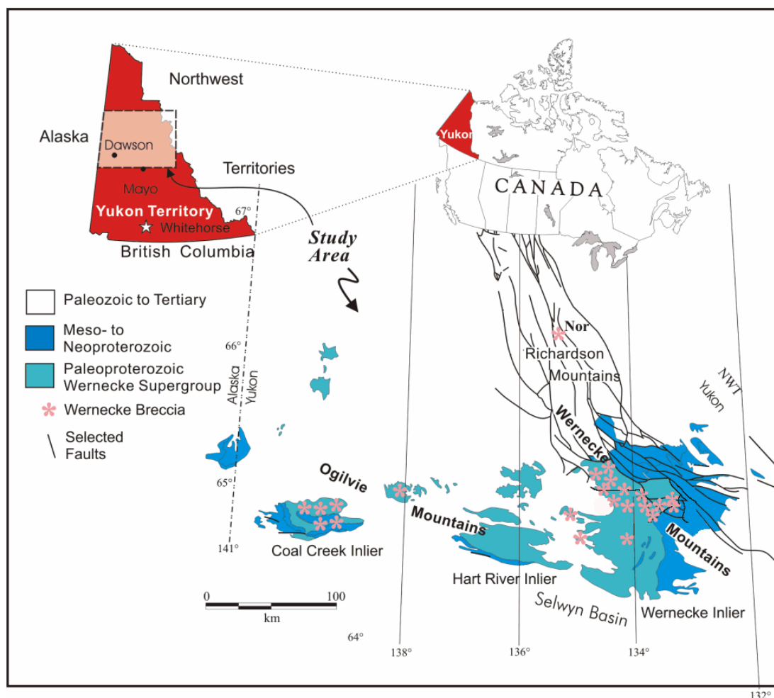
Figure 1: Regional location and geological setting of the Wernecke district.
