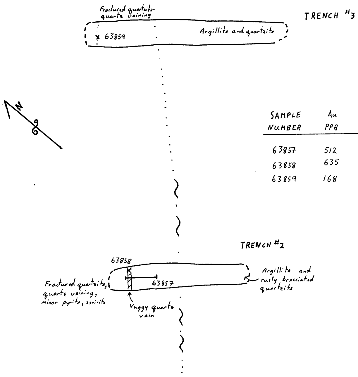
Figure 7: TRENCH PLAN
